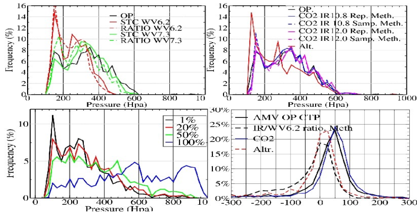
Figure 4: CTP distribution for (left top panel) the four WV/IR retrievals, (right top) the four CO2/IR retrievals, (left bottom panel) for several CALIOP representative CTP's. In top panels are also given the operational CTP curve (black curve), in right-top panel is given the alternative CTP (red curve). In the bottom-right panel, distribution of AMV CTP minus CALIOP CTP (percentil 20) for the AMV OP meth., IR/WV6.2 ratio meth, CO2 meth., ALT meth.
