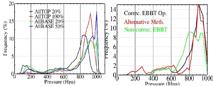
Figure 5: Distributions of CTP for : (left panel) CALIOP AllTOP at percentile 20 and 100 and CALIOP All BASE at percentile 20 and 50 CTP , (right panel) the AMV and the operational method, the alternative method and the operational AMV before correction for low clouds.
