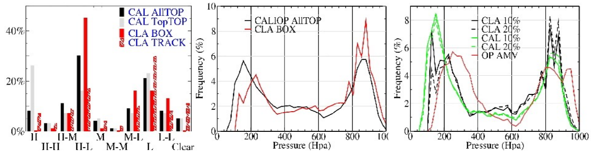
Figure 2: distribution of the 10 cloud types for CLA BOX , CLA track, CAL TopTOP and AllTOP (left), CLA BOX and CAL ALLTOP CTP distributions (middle) etcet).
