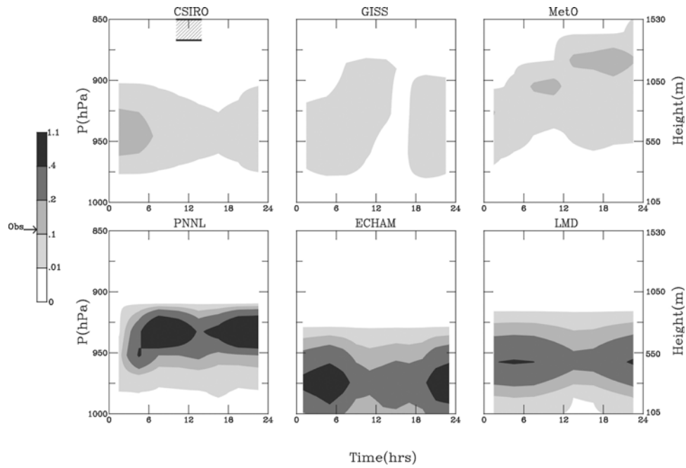
Figure 4a. Similar to Figure 1a but for cloud water mixing ratio (g/kg). Observed values are also indicated on the color bar.
