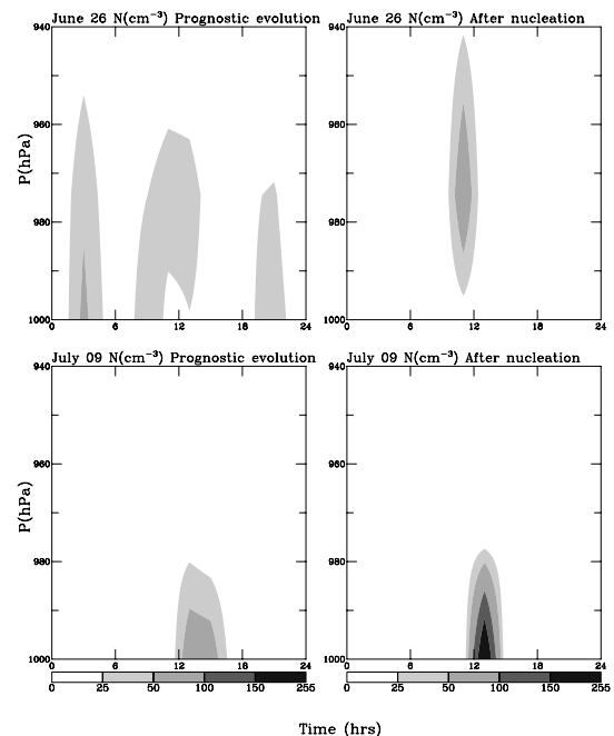
Figure 6. Time-pressure plot of the ECHAM simulation of cloud droplet number concentration ( N ) that shows the differences in N when N is treated prognostically and when N is calculated right after nucleation for the clean (26 June) and the polluted case (9 July).
