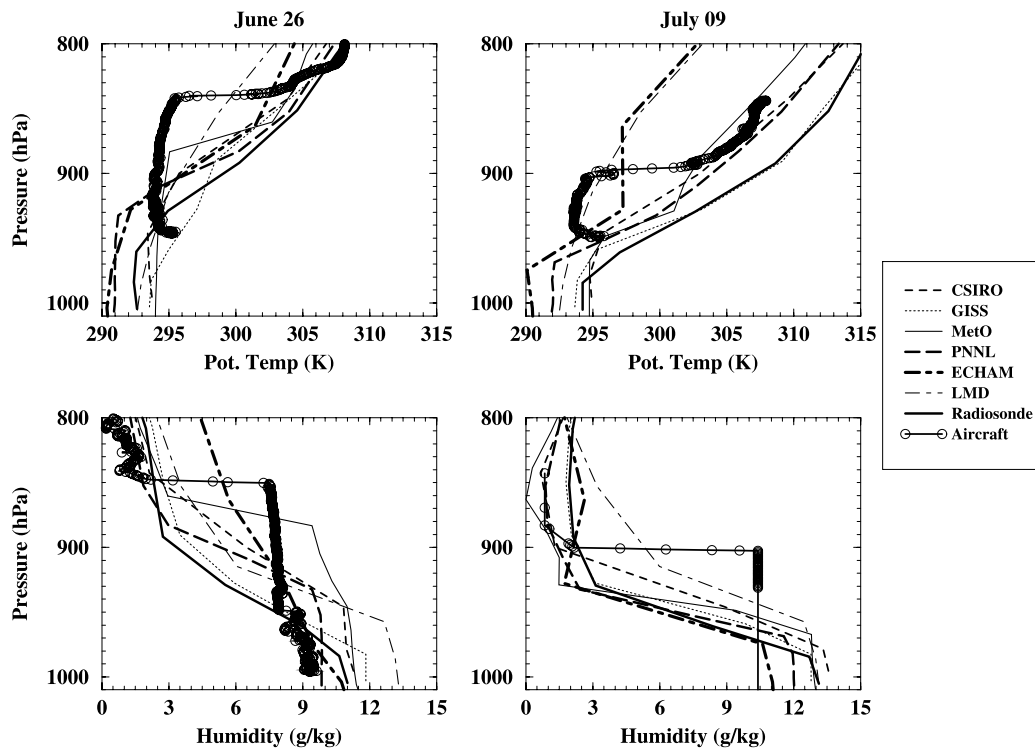
Figure 3. Potential temperature ( T ) and humidity ( q_v ) soundings from the 6 SCMs, aircraft data, and radiosonde for the clean and polluted case at 12Z.
