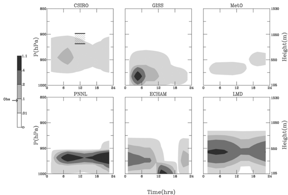
Figure 4b. Similar to Figure 4a but for the polluted case (9 July).
