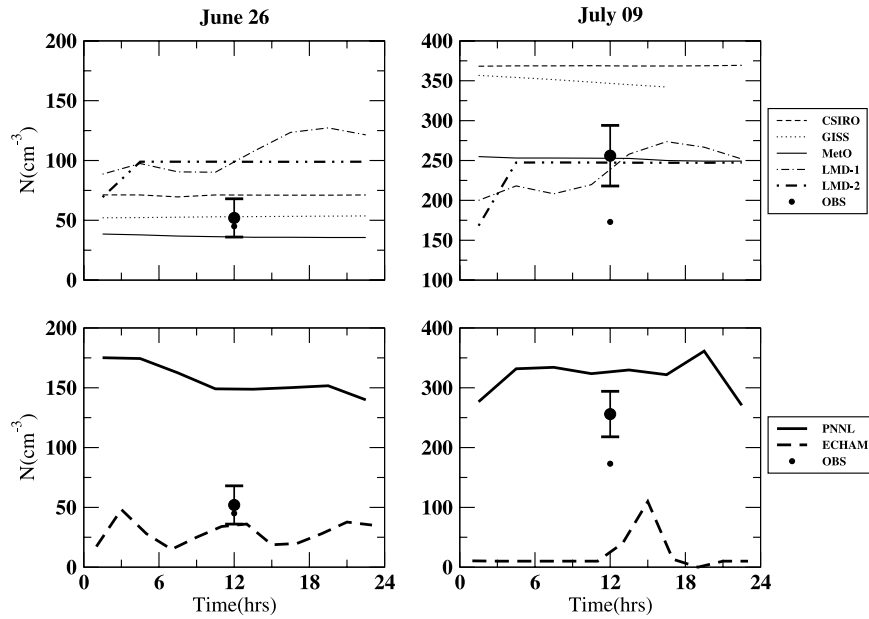
Figure 5. Time series of predicted cloud droplet number concentration ( N ) for the clean and polluted cases for the diagnostic (upper panels) and prognostic (lower panels) schemes. Observations, plotted at 12 Z, are from in situ measurements averaged from 12 Z to 15 Z. For observed N , two values are indicated: N for selective sampling and representative of aerosol impacts on clouds as described in Section 2.1 and the average N for all conditions (including mixing and scavenging) that have lower values of 45 \text{ cm}^{-3} and 173 \text{ cm}^{-3} for June 26 and July 9, respectively. Two values for LMD are N predicted from simulated aerosol mass (LMD-1) and N predicted from observed aerosol mass (LMD-2).
