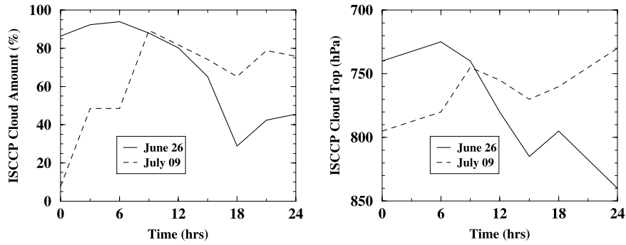
Figure 2. Time series of ISCCP retrieved cloud amount and cloud top levels for the clean (26 June) and the polluted case (9 July).
