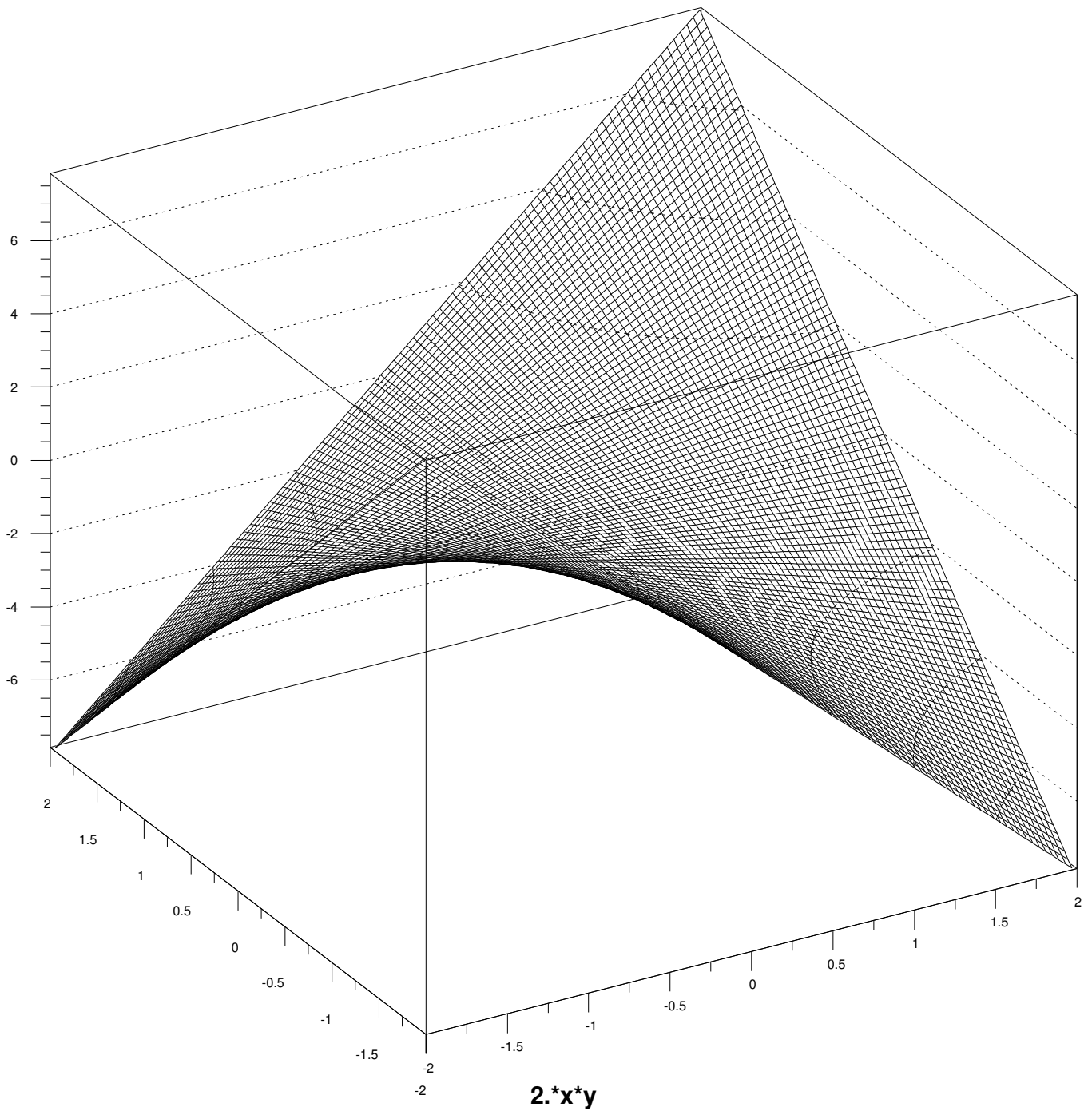
FIGURE 2 – Partie imaginaire de z^2 ( = 2xy )
