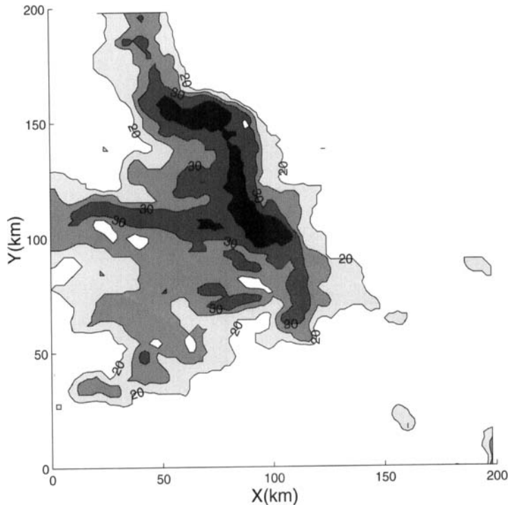
Figure 1. Horizontal cross-section of airborne radar reflectivity (dBZ) at 2215 UTC 22 February 1993 at a height of 500 m over a domain of 200 km \times 200 km.
