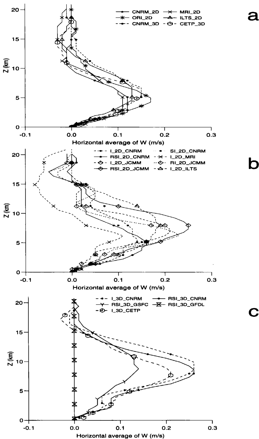
Figure 14. Vertical profiles of vertical velocity ( \text{m s}^{-1} ) averaged from 5 to 6 hours of (a) the 2D and 3D cloud-resolving model (CRM) simulations with no ice-phase parametrization, (b) the 2D CRM simulations with an ice-phase parametrization, and (c) the 3D CRM simulations with an ice-phase parametrization (see Tables 1 and 4 for an explanation of the acronyms).
