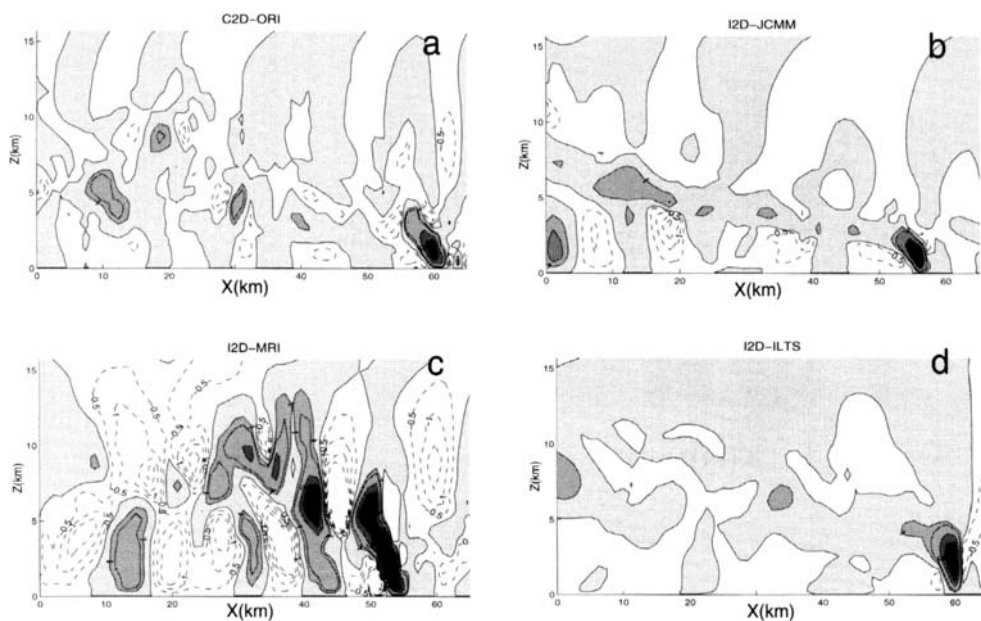
Figure 10. Vertical cross-sections of the vertical velocity ( \text{m s}^{-1} , contour interval 1 \text{ m s}^{-1} ) after 6 hours run time for runs (a) C2D (ORI), (b) I2D (JCMM), (c) I2D (MRI), (d) I2D (ILTS), (e) I2D (CNRM), (f) RSI3D (GFDL), (g) RSI3D (CNRM), (h) RSI3D (GSFC), and (i) I3D (CETP)—only part of the simulation domain is shown (see Tables 1 and 4 for an explanation of the acronyms).
