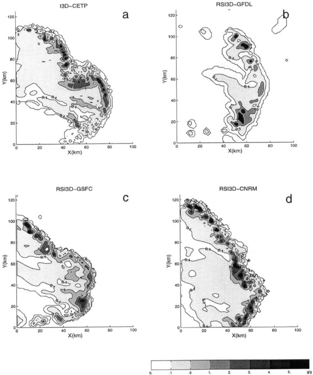
Figure 7. Horizontal cross-sections of the total hydrometeor fields (contour interval 1.0 \text{ g kg}^{-1} , except that the first two isolines correspond to values of 0.1 and 0.5 \text{ g kg}^{-1} ) after 6 hours run time and at a height of 1.4 \text{ km} for runs (a) I3D (CETP), (b) RSI3D (GFDL), (c) RSI3D (GSFC), and (d) RSI3D (CNRM) (see Tables 1 and 4 for an explanation of the acronyms).
