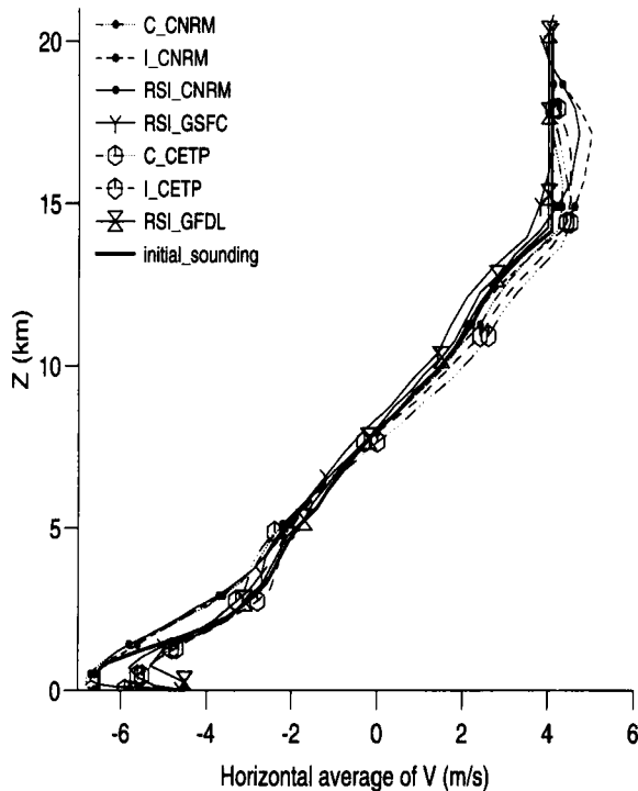
Figure 13. Vertical profiles of the v (squall-line parallel) component of the wind ( \text{m s}^{-1} ) averaged from 5 to 6 h of the 3D cloud-resolving simulations (see Tables 1 and 4 for an explanation of the acronyms).
