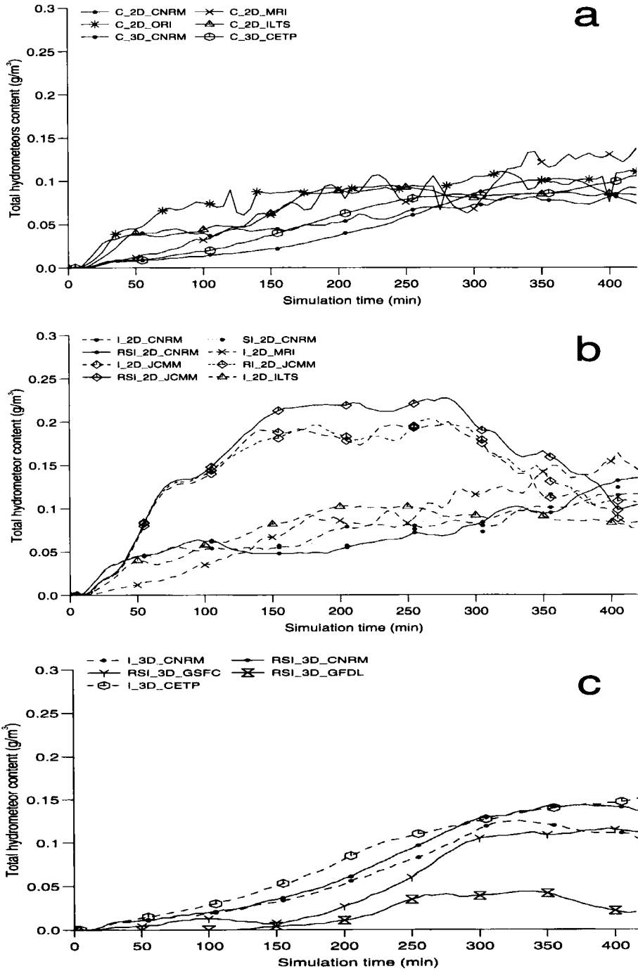
Figure 6. As Fig. 4, but for the domain-averaged total hydrometeor (liquid + solid) water content ( \text{g m}^{-3} ).
