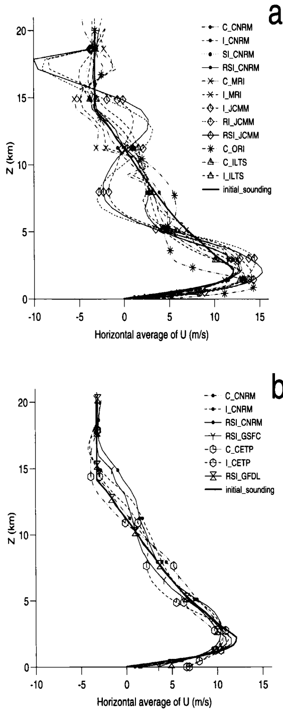
Figure 12. Vertical profiles of the u (squall-line normal) component of the wind ( \text{m s}^{-1} ) averaged from 5 to 6 h of (a) the 2D cloud-resolving model (CRM) simulations, and (b) the 3D CRM simulations (see Tables 1 and 4 for an explanation of the acronyms).
