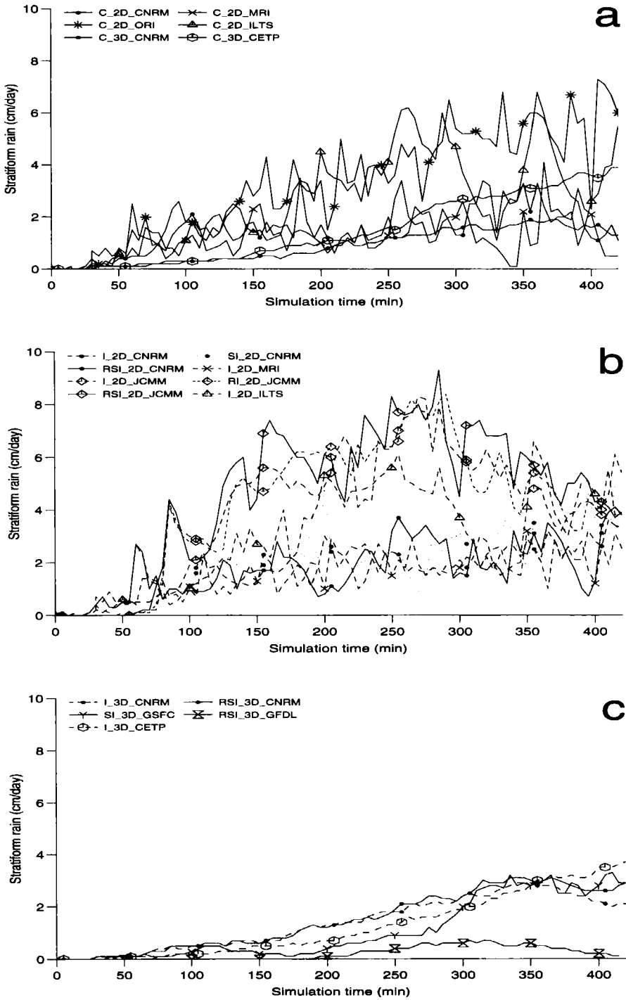
Figure 5. As Fig. 4, but for the stratiform surface rain rate ( \text{cm day}^{-1} ).
