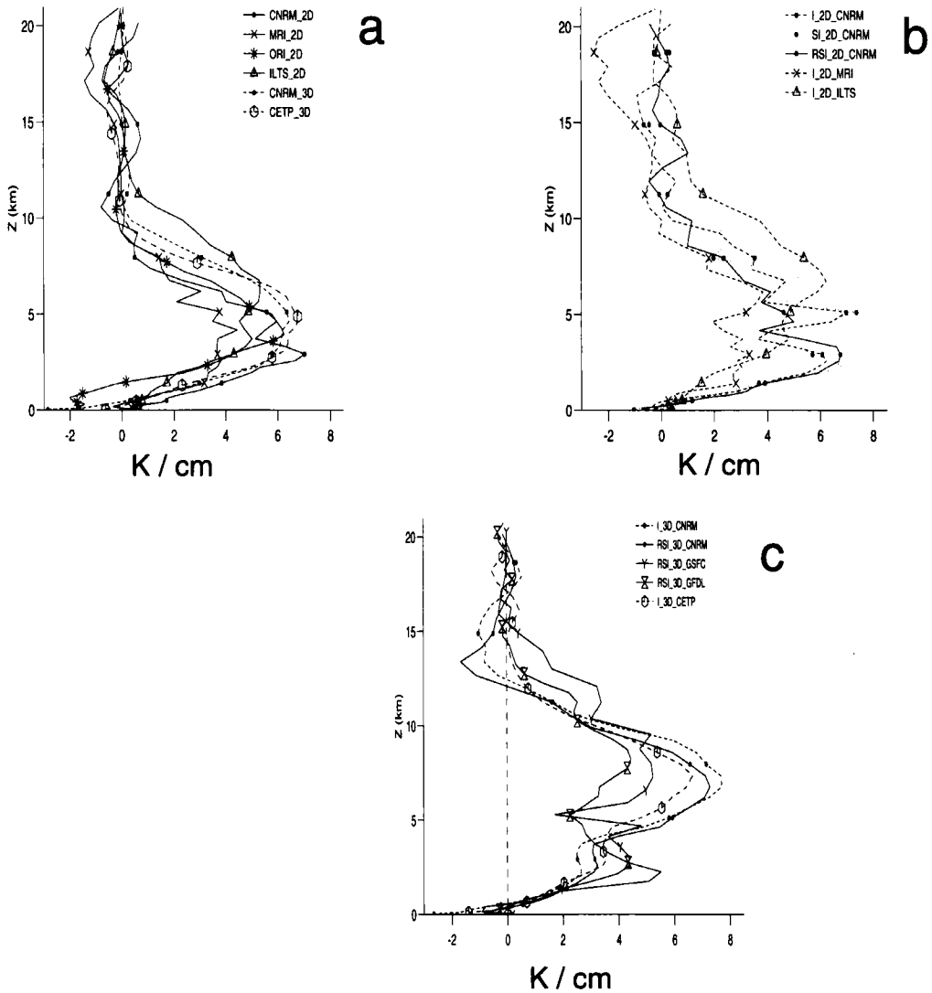
Figure 18. As Fig. 14, but for the apparent heat source normalized by the total surface rainfall ( K\text{ cm}^{-1} ).
