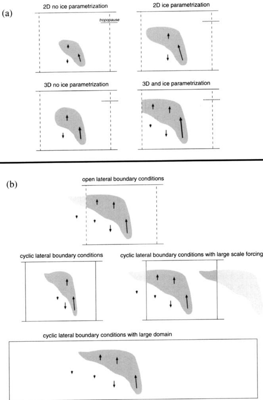
Figure 22. Schematic diagram showing the impact of (a) the dimensionality and ice-phase parametrization, and (b) the lateral boundary conditions (arrows indicate the mean vertical motion).
