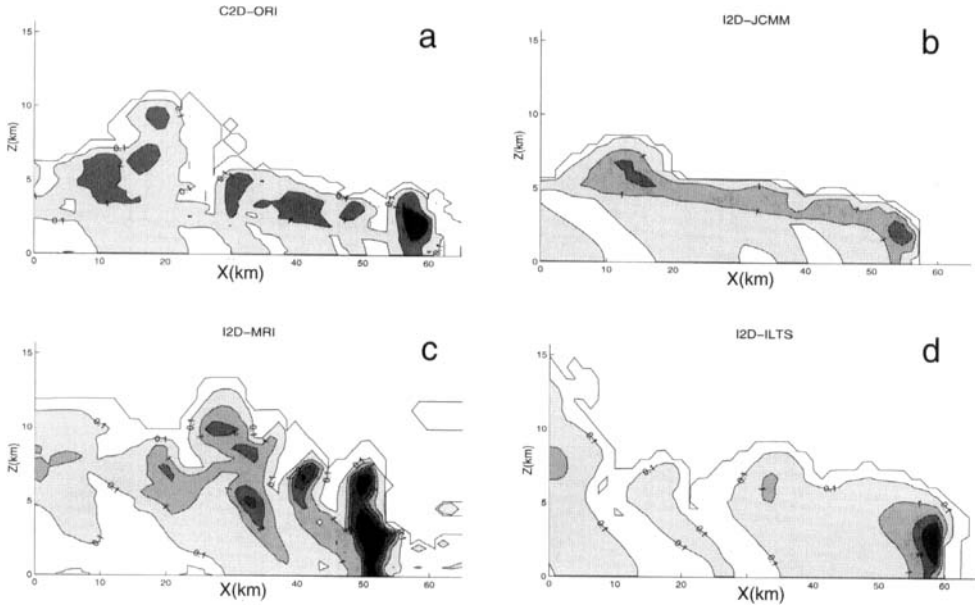
Figure 11. As Fig. 10, but for the total hydrometeor (liquid + solid) fields ( \text{g kg}^{-1} , contour interval 1.0 \text{ g kg}^{-1} , except that the first two isolines correspond to values of 0.1 and 0.5 \text{ g kg}^{-1} ).
