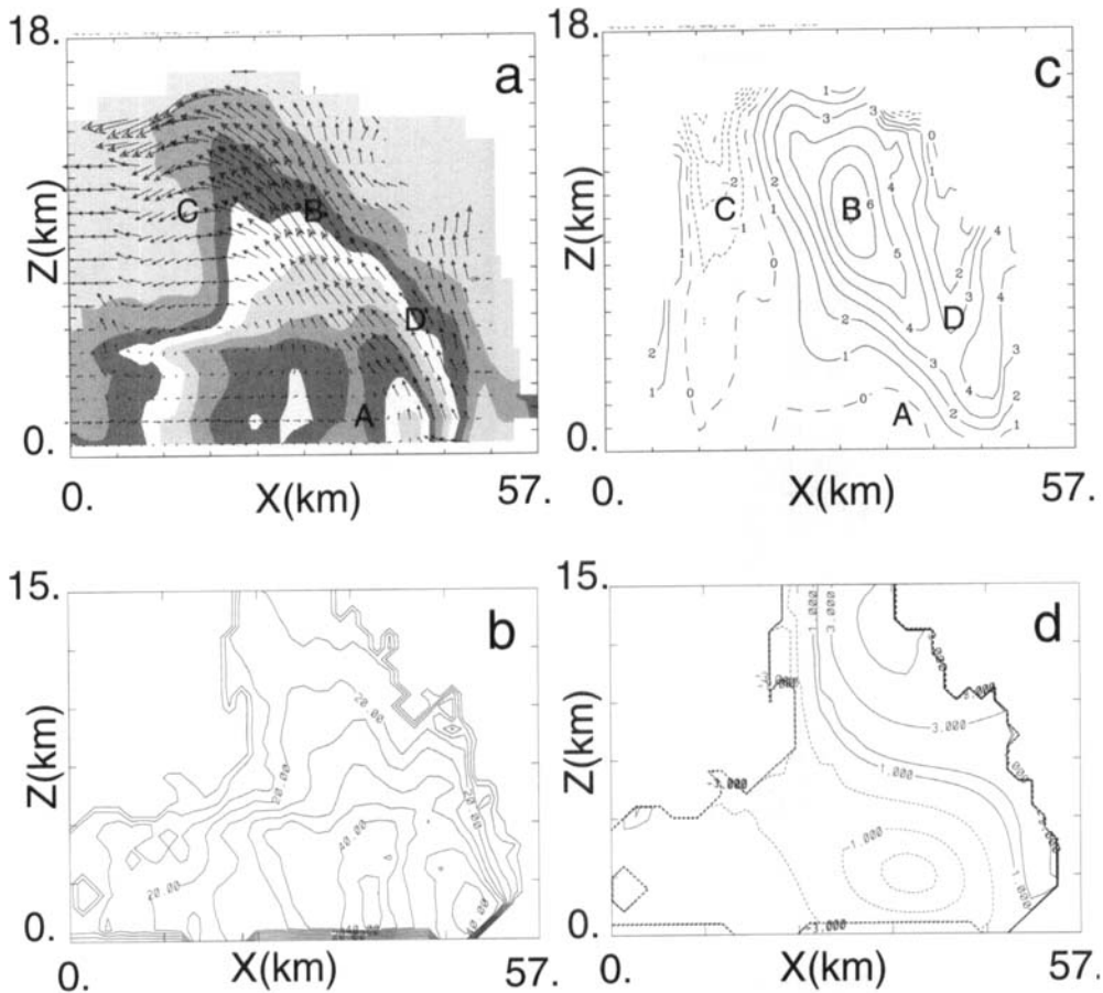
Figure 9. Vertical cross-sections (a) and (b) of radar reflectivity (dBZ, contour interval 5 dBZ), and (c) and (d) of vertical velocity ( \text{m s}^{-1} , contour interval 1 \text{ m s}^{-1} ) as analysed from Doppler radar observations around 2100 UTC 22 February 1993 over domains (a) and (c) 57 \text{ km} \times 18 \text{ km} constructed from 40 km averages along the squall line (Jorgensen et al. 1997), and (b) and (d) 57 \text{ km} \times 15 \text{ km} constructed from 7 km averages along the squall line (Montmerle and Lemaitre 1998). Doppler wind arrows are shown in (a).
