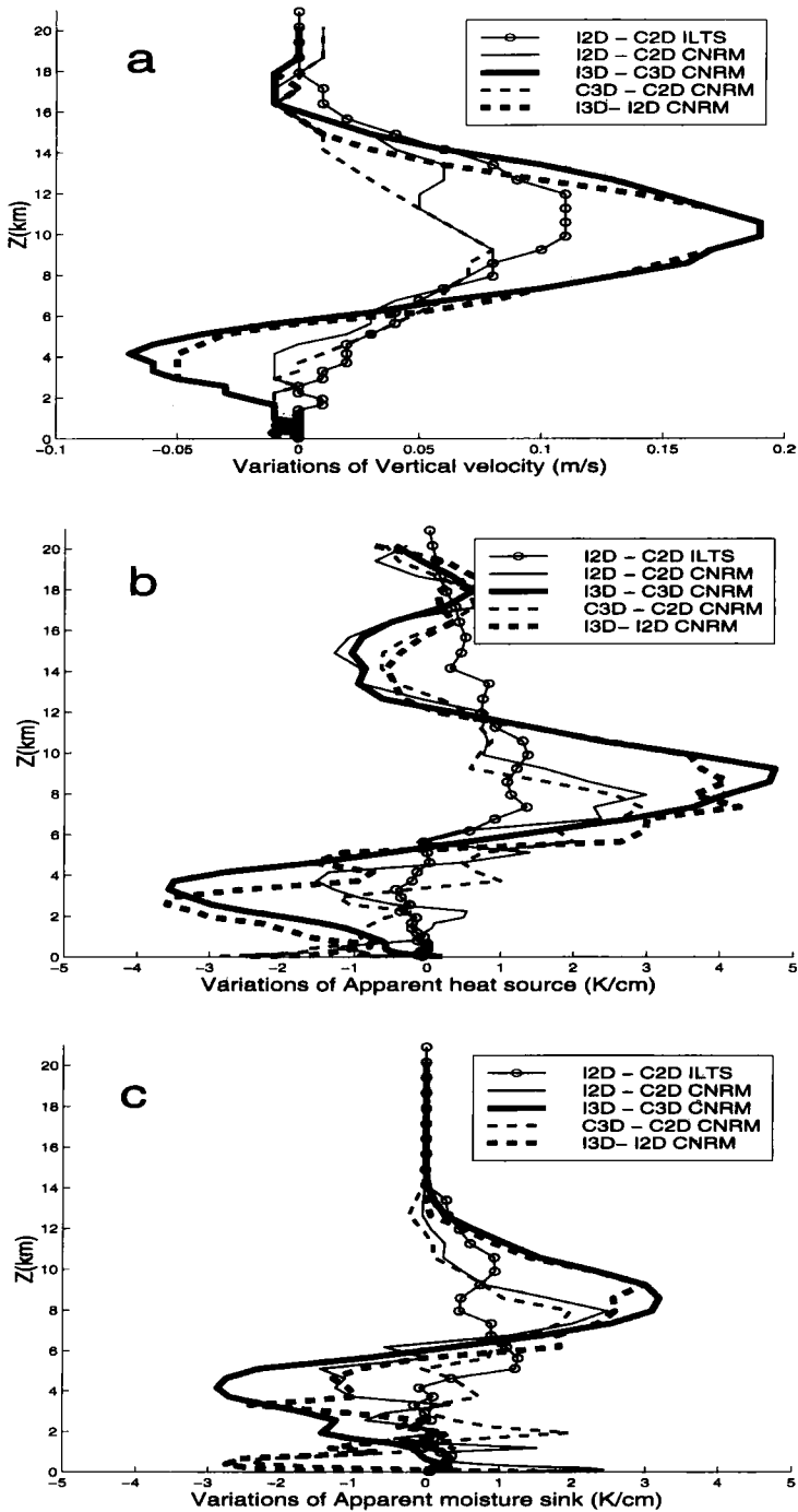
Figure 15. Differences between experiments illustrating the effects of ice-phase parametrizations and dimensionality. (a) The vertical velocity ( \text{m s}^{-1} ), (b) the apparent heat source normalized by the total surface rainfall ( \text{K cm}^{-1} ), and (c) the apparent moisture sink normalized by the total surface rainfall ( \text{K cm}^{-1} ). The solid lines show the differences between experiments with and without an ice-phase parametrization, and the dashed lines show the differences between the 3D and 2D experiments (see Tables 1 and 4 for an explanation of the acronyms).
