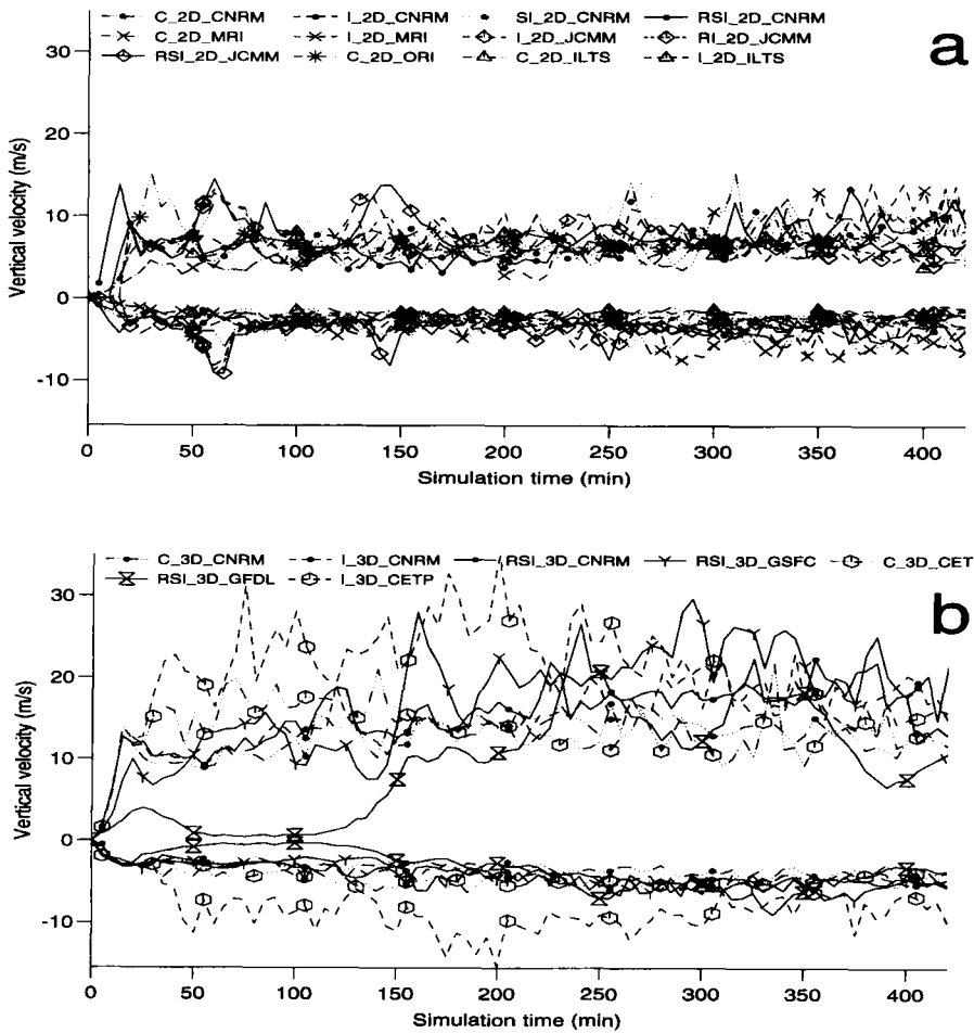
Figure 3. Time history of the maximum and minimum vertical velocity ( \text{m s}^{-1} ) for (a) the 2D cloud-resolving models, and (b) the 3D cloud-resolving models (see Tables 1 and 4 for an explanation of the acronyms).
