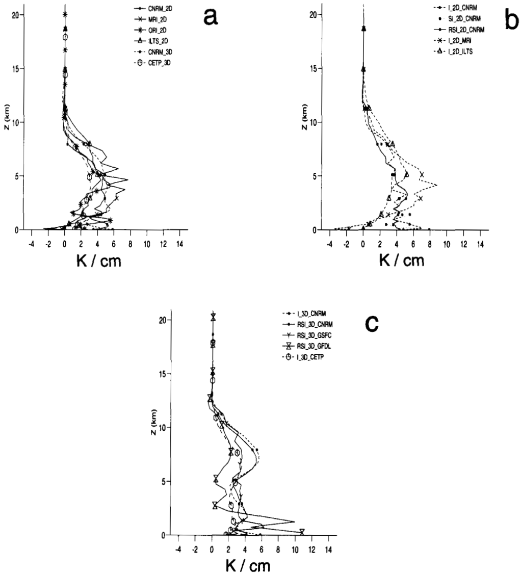
Figure 19. As Fig. 14, but for the apparent moisture sink normalized by the total surface rainfall ( K\text{ cm}^{-1} ).
