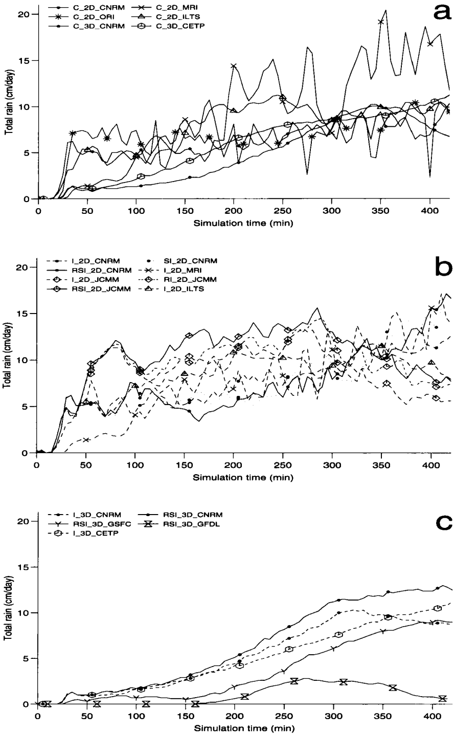
Figure 4. Time history of the total surface rain rate ( \text{cm day}^{-1} ) for (a) the 2D and 3D cloud-resolving models (CRMs) with no ice-phase parametrization, (b) the 2D CRMs with an ice-phase parametrization, and (c) the 3D CRMs with an ice-phase parametrization (see Tables 1 and 4 for an explanation of the acronyms).
