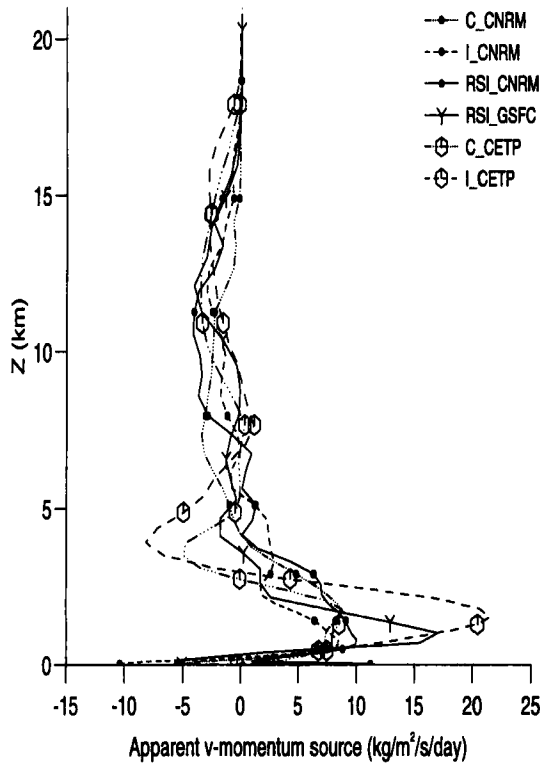
Figure 21. The vertical profiles of v (squall-line parallel) momentum source ( \text{kg m}^{-2}\text{s}^{-1}\text{day}^{-1} ) averaged from 5 to 6 hours of the 3D cloud-resolving model (CRM) simulations (see Tables 1 and 4 for an explanation of the acronyms).
