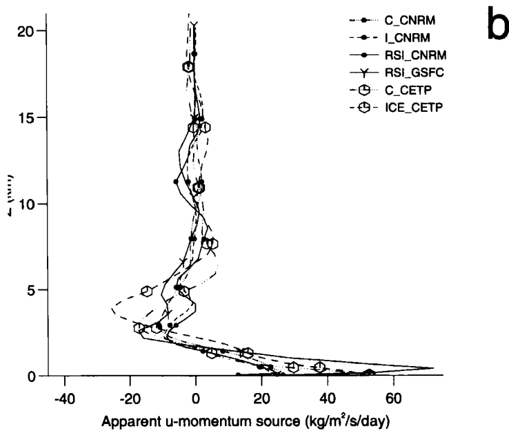
Figure 20. The vertical profiles of the u (squall-line normal) momentum source ( \text{kg m}^{-2}\text{s}^{-1}\text{day}^{-1} ) averaged from 5 to 6 hours of (a) the 2D cloud-resolving model (CRM) simulations, and (b) 3D CRM simulations (see Tables 1 and 4 for an explanation of the acronyms).
