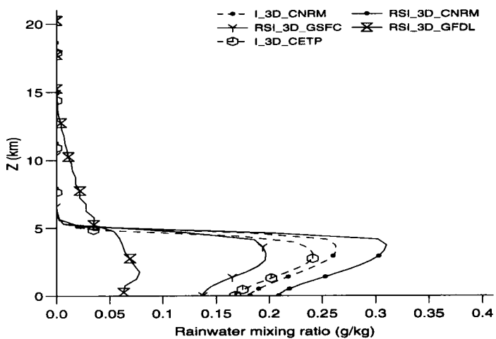
Figure 16. As in Fig. 14, but for the rain water content ( \text{g kg}^{-1} ).
