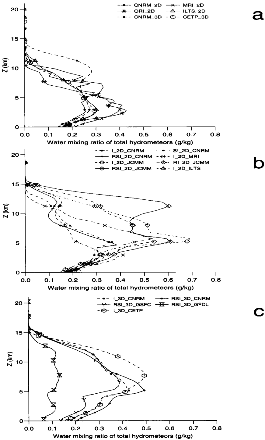
Figure 17. As in Fig. 14, but for the total water content (liquid + solid) ( \text{g kg}^{-1} ).
