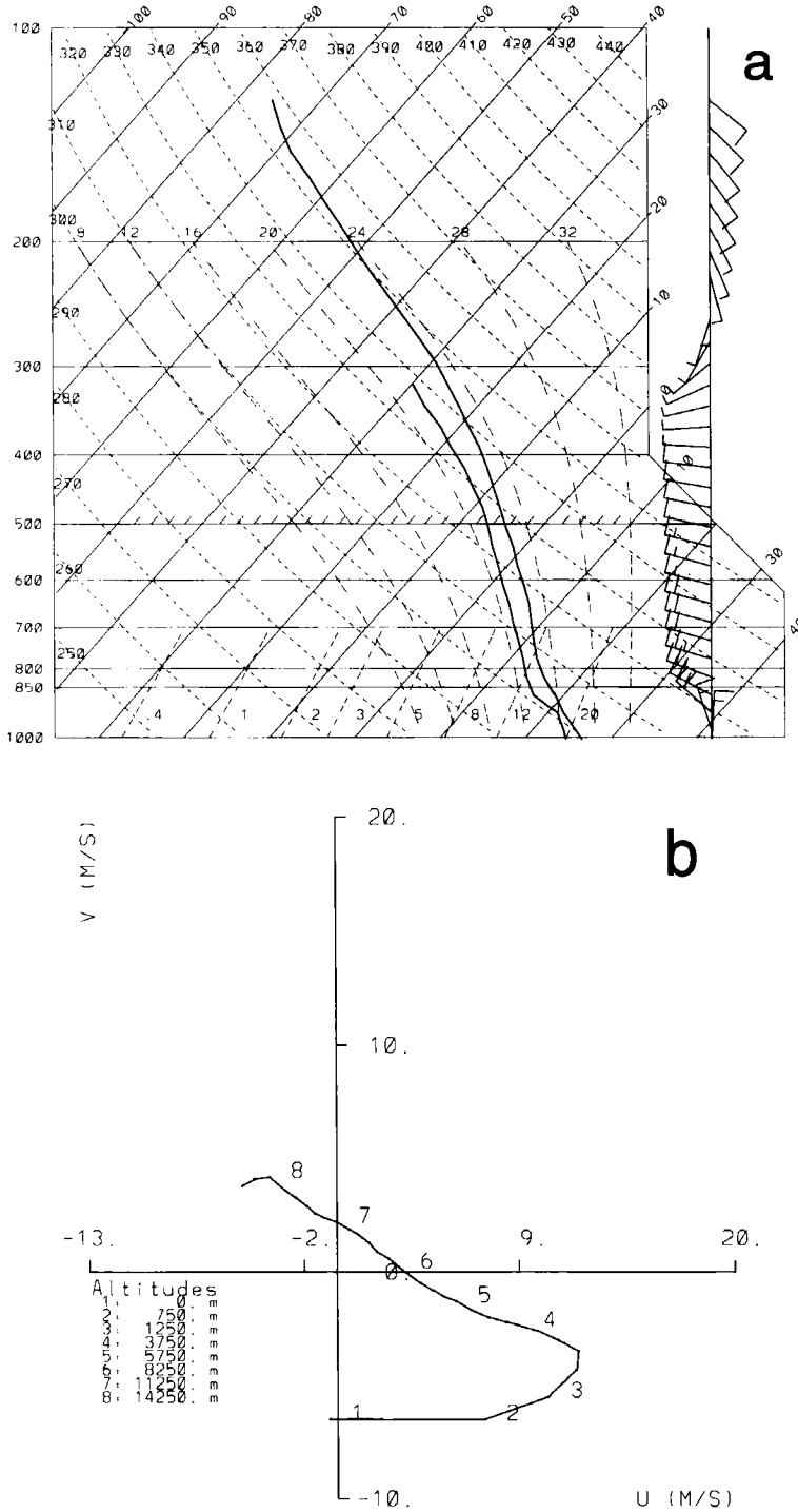
Figure 2. Specified initial conditions for the model runs. (a) Temperature and specific humidity plotted on a skew- T log- P diagram and (b) the horizontal wind components ( U positive towards the east and V positive towards the north) plotted on a hodograph—data courtesy of M. A. LeMone.
