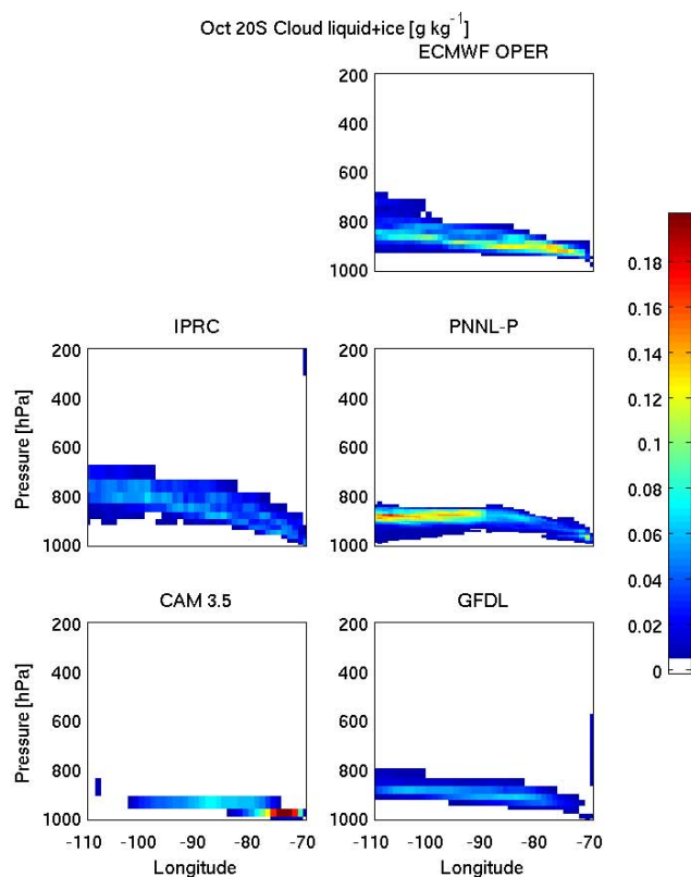
Fig. 9. October 2006 mean 20^\circ\text{S} cross sections of model liquid water content ( \text{g kg}^{-1} ).
