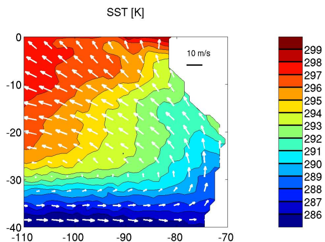
Fig. 1. October 2006 mean AMSR-E SST(K) and QuikSCAT winds ( 10 \text{ ms}^{-1} scale plotted).
