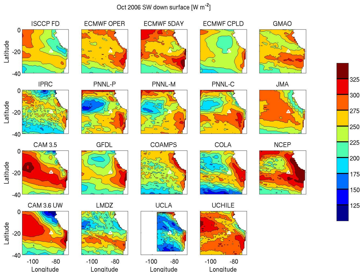
Fig. 6. October 2006 mean downwelling SW radiation at the surface from ISSCP and models ( \text{W m}^{-2} ).
