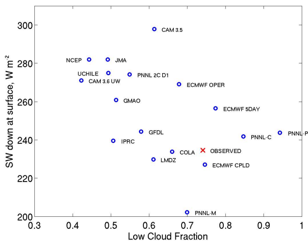
Fig. 7. Mean October 2006 downwelling shortwave radiation at the surface versus low cloud fraction for a 5^\circ \times 5^\circ box centered at 85^\circ \text{W} 20^\circ \text{S} . The observed value (red x) comes from ISSCP FD data and MODIS liquid cloud fraction.
