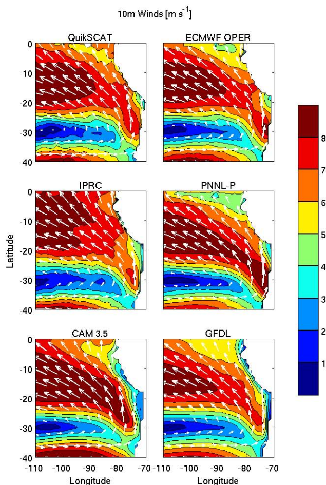
Fig. 2. October 2006 mean 10-m wind speed ( \text{ms}^{-1} ) and wind vectors for QuikSCAT (upper left) and a selection of models.
