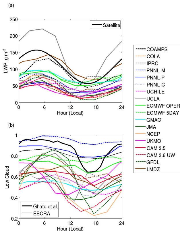
Fig. 11. Composite October 2006 diurnal cycle of (a) liquid water path ( \text{g m}^{-2} ) and (b) low cloud fraction at the IMET buoy at 85° W 20° S. In (a) satellite observations from 2006 (see text) are plotted (thick black line) and in (b) observed climatologies of cloud fraction from the buoy (Ghate et al., 2009, thick black line) and EECRA (Hahn and Warren, 1999, thin black line) are plotted.
