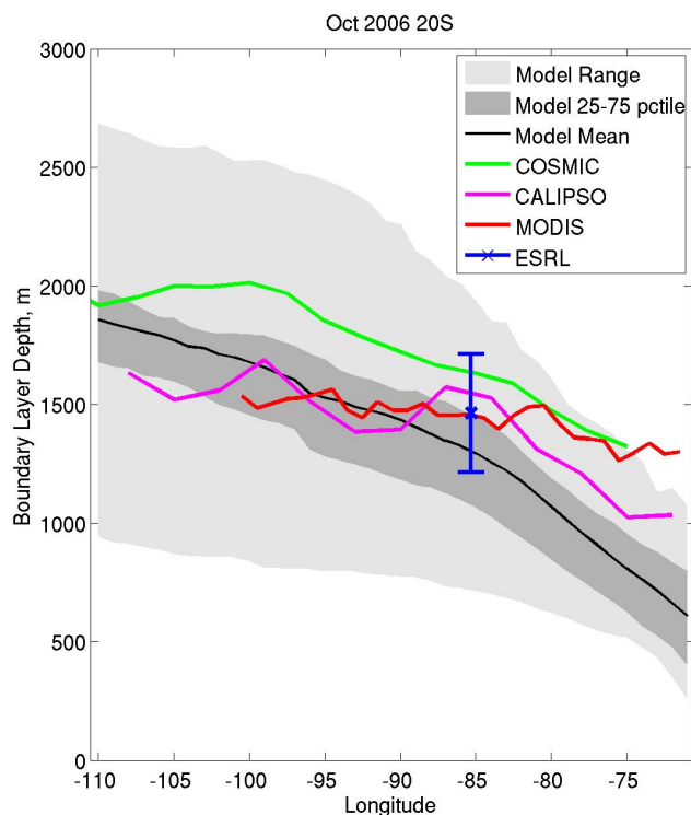
Fig. 10. October 2006 model boundary layer depth (m) compared with observations of boundary layer depth and cloud-top height. Model mean (solid black line), 25–75 percentile range (dark gray), and model range (light gray) are plotted. COSMIC October 2006 boundary layer depth sampled over 15–25° S is plotted in green. CALIPSO cloud-top height is plotted in magenta. MODIS cloud-top heights are plotted in red from Zuidema et al. (2009). The mean depth (blue x) is an October climatology estimated from NOAA/ESRL soundings taken near the stratus buoy, with standard deviation plotted.
