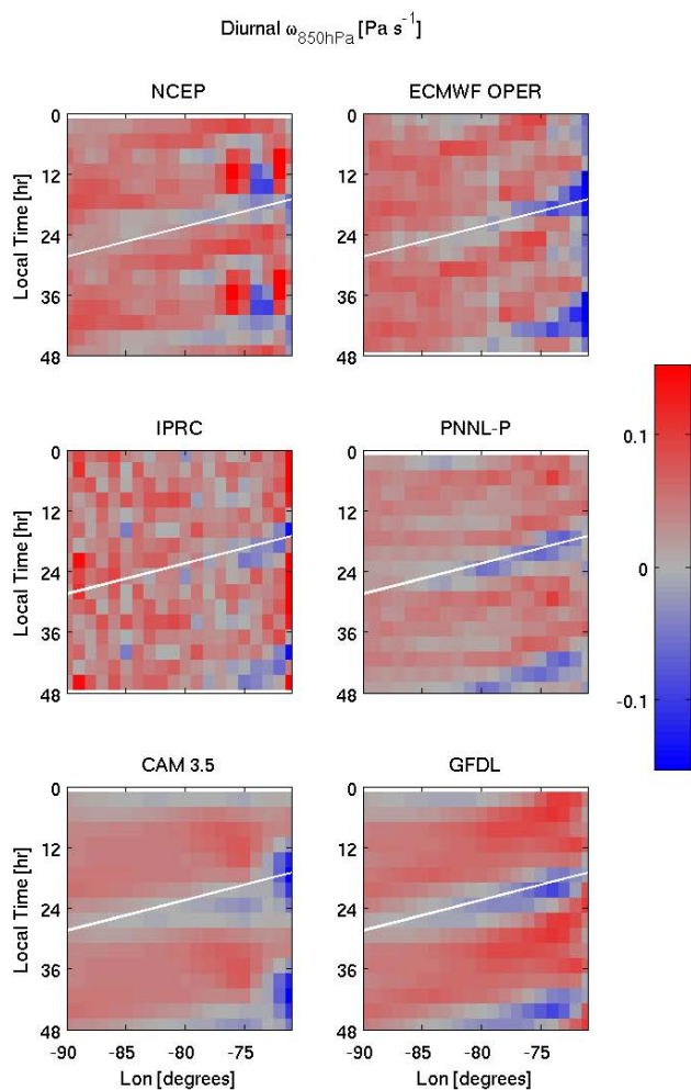
Fig. 12. Hovmöller diagram along 20^{\circ} S of a 24-h composite (repeated twice for clarity) of omega at 850 hPa ( \text{Pa s}^{-1} ) of selected models for October 2006. White line is phase speed of 30 \text{ ms}^{-1} .
