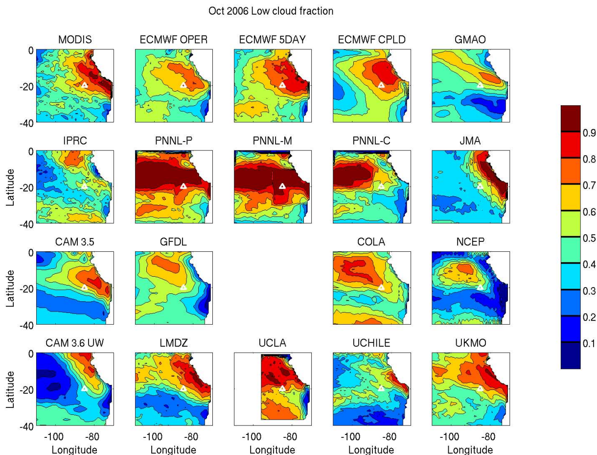
Fig. 4. October 2006 MODIS total cloud fraction (upper left) and modeled monthly-mean low-cloud fraction.
