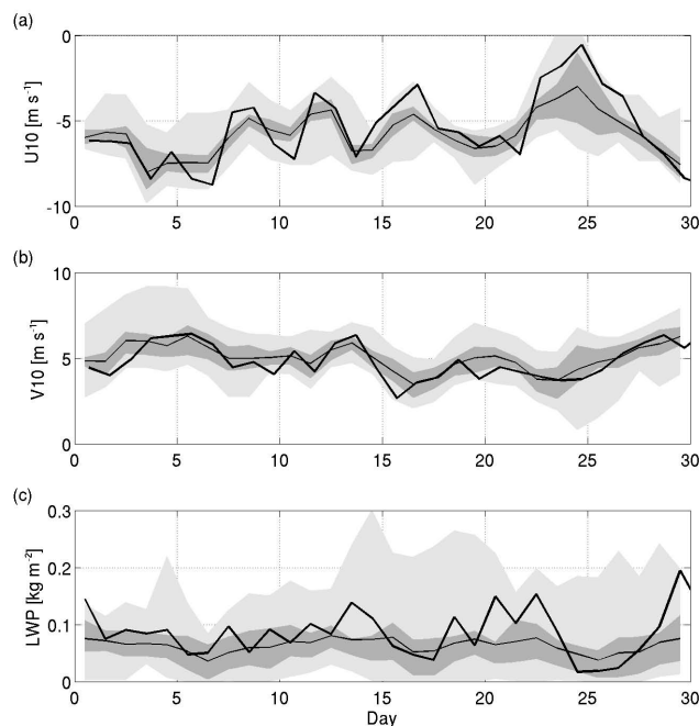
Fig. 13. Time series of 24-h averaged (a) 10-m zonal velocity ( \text{ms}^{-1} ), (b) 10-m meridional velocity ( \text{ms}^{-1} ), and (c) liquid water path ( \text{kg m}^{-2} ) for a 3^{\circ} \times 3^{\circ} box centered at 20^{\circ} S 85^{\circ} W. Model means (light black line), 25th–75th percentile range (dark gray), and model range (light gray) are plotted. Heavy black lines indicate observations; QuikSCAT in (a) and (b) and AMSR-E LWP in (c), respectively. Day 0 on the time axis corresponds to 0 Z, 1 October 2006.
