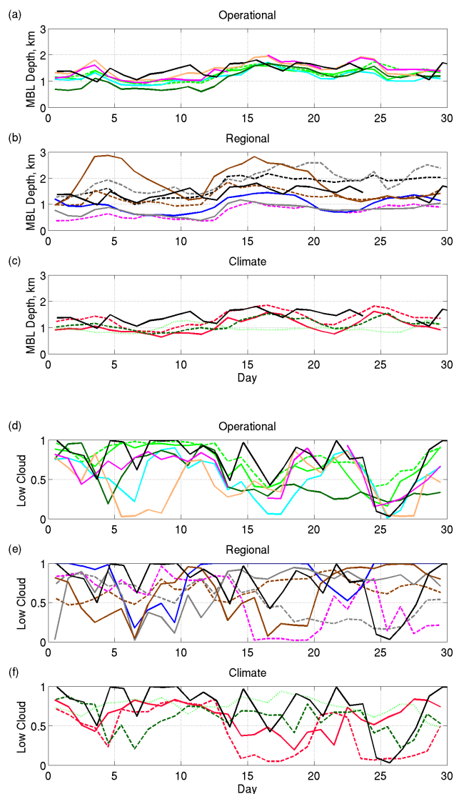
Fig. 15. October 2006 time series of 24-h mean boundary layer depth in km (a–c) and low cloud fraction (d–f) for a 3^\circ \times 3^\circ box centered at 20^\circ S 85^\circ W. Solid black lines are MODIS cloud-top height and MODIS cloud fraction. Model line types as in Fig. 8.
