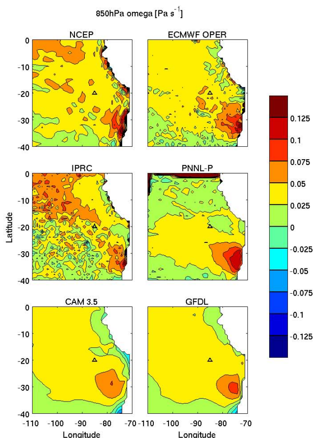
Fig. 3. October 2006 mean subsidence at 850 hPa ( \text{Pa s}^{-1} ). NCEP and ECMWF analysis is shown in lieu of observed subsidence. The stratus buoy location is indicated with a triangle.
