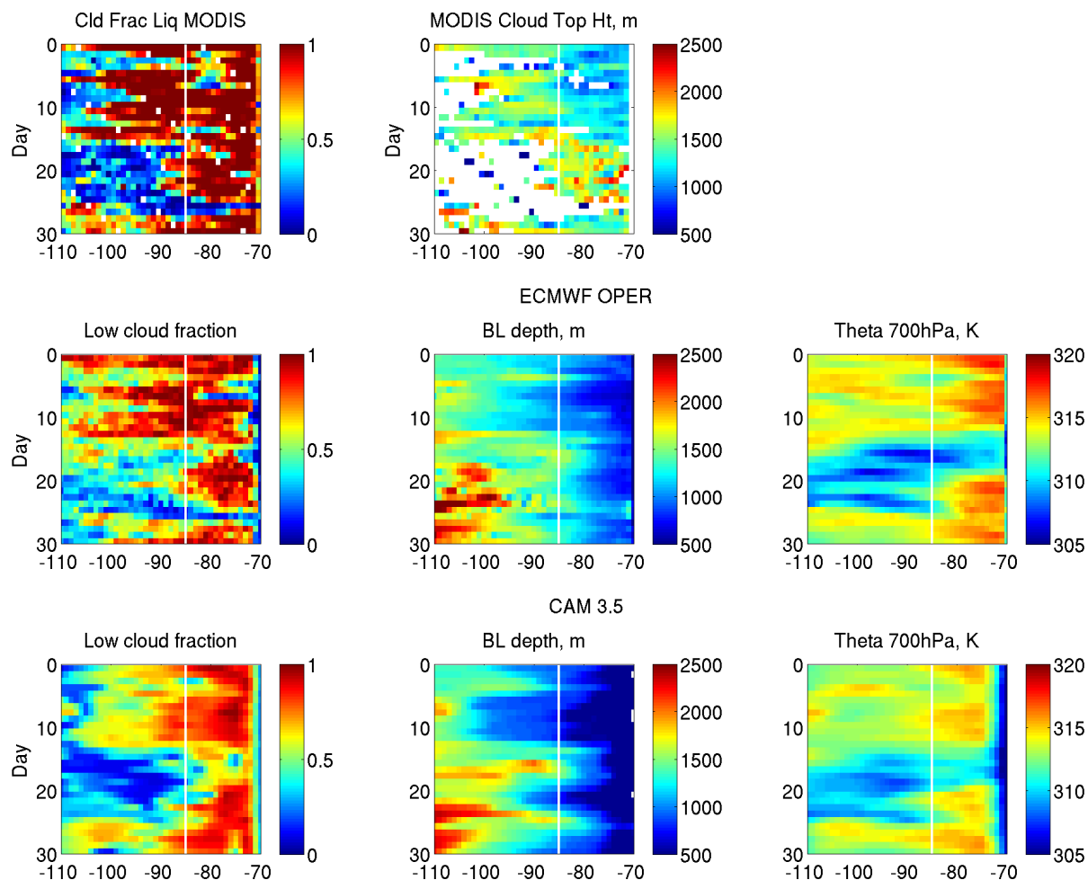
Fig. 14. Hovmöller diagrams of 24-h means along 20^{\circ} S for October 2006. MODIS cloud fraction and cloud top height (m) are plotted in the top row. The bottom two rows are low cloud fraction, boundary layer depth (m), and potential temperature at 700 hPa (K) for the ECMWF operational model and CAM 3.5, respectively. The white line indicates the stratus buoy position. All data are horizontally averaged over a 1^{\circ} \times 1^{\circ} box.
