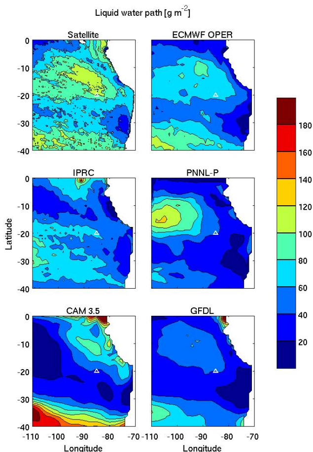
Fig. 5. October 2006 mean satellite liquid water path (upper left, \text{gm}^{-2} ) and modeled liquid water path ( \text{gm}^{-2} ).
