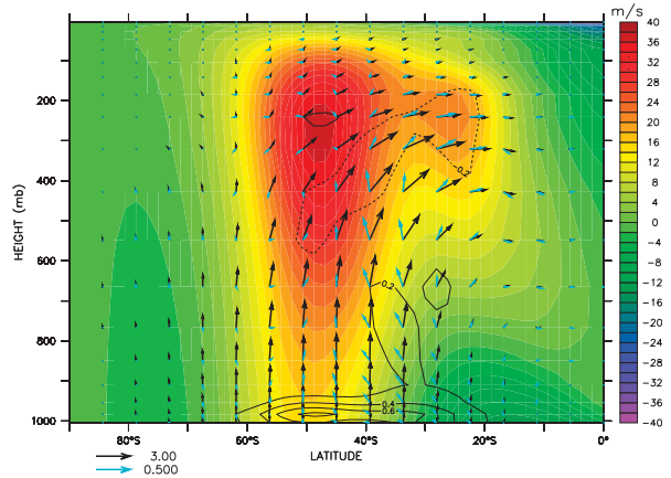
b) Eliassen-Palm fluxes ( 144 \times 96 - 96 \times 96 )
