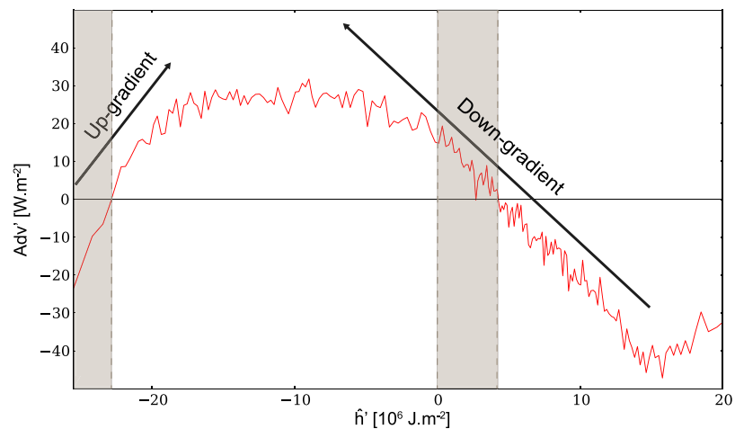
Figure 7. Advection anomaly ( Adv' ) as a function of h' calculated over the same region as in Figure 4 during the initiation period. Both terms are integrated over the troposphere. Grey shading indicates a positive feedback of h' Adv' (equation (3)) while areas without shading indicate h' Adv' < 0 , showing the dominance of the negative feedback. Dry regions correspond to h' < 0 and moist regions to h' > 0 .
