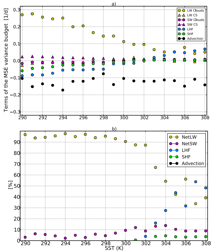
Figure 3. (a) LW (yellow) and SW (pink) due to clouds (circles) or clear sky (triangles), LHF (blue), SHF (green), and advection (black) covariance terms of equation (3) for SSTs between 290 and 308 K. Shown are averages for the initiation period. (b) Relative proportion of positive feedbacks on self-aggregation as a function of SST over the same period. NetLW and NetSW correspond to the total (clear sky and clouds) LW and SW terms.
