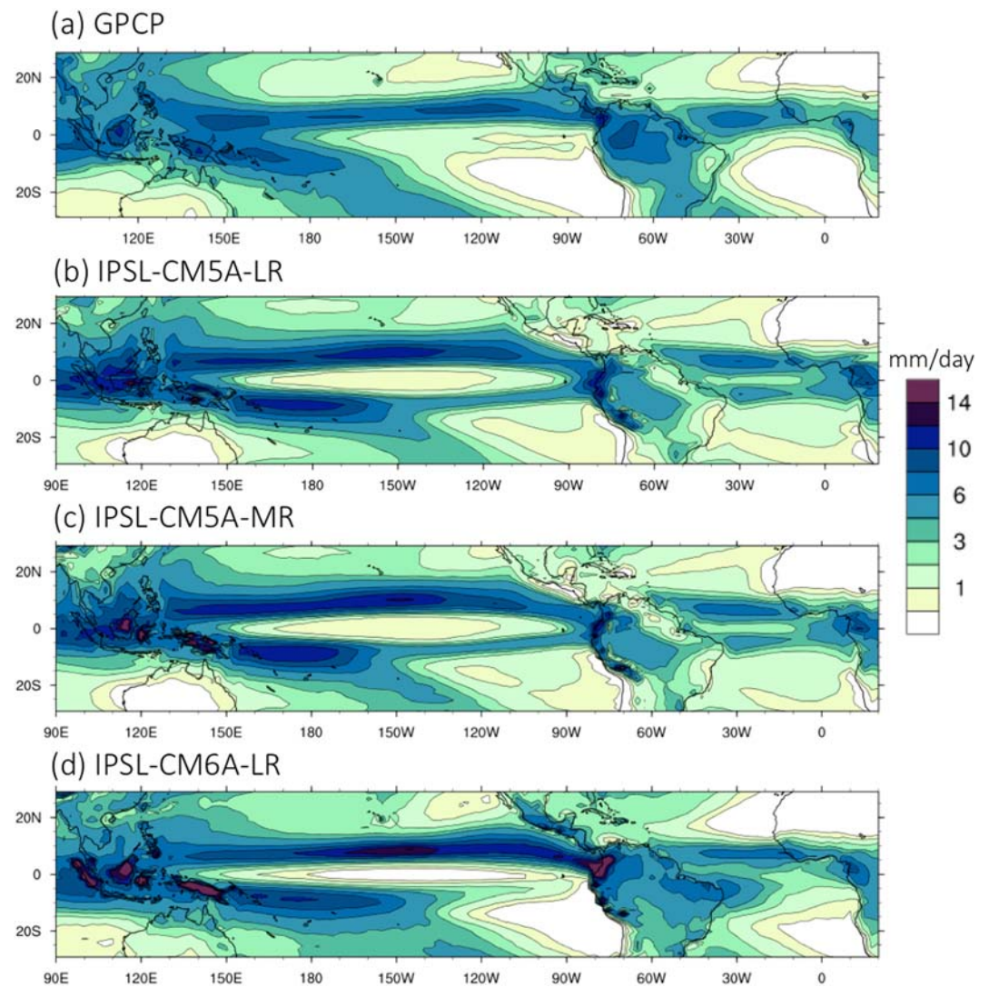
Figure 6. Annual mean precipitation rate (in mm day -1 ) for (a) GPCP, (b) IPSL-CM5A-LR, (c) IPSL-CM5A-MR, and (d) IPSL-CM6A-LR in the tropical region. The climatology is computed over the 1980–2005 period for the models and 1980–2009 for GPCP (Adler et al., 2018).
