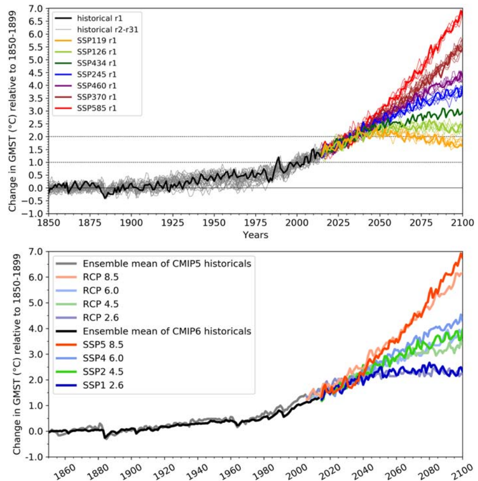
Figure 31. (upper panel) Change in global mean surface air temperature (GMST, in °C) relative to the 1850–1899 period in the historical r1i1p1f1 member (thick black line) and the other members (thin gray lines) and scenario experiments for the r1i1p1f1 member (thick colored lines) and other members (thin colored lines). Anomalies for 0°C, 1°C, and 2°C are indicated for reference. (lower panel) change in GMST relative to the 1850–1899 period for the IPSL-CM5A-LR and IPSL-CM6A-LR models for the historical period and the 21st century.
