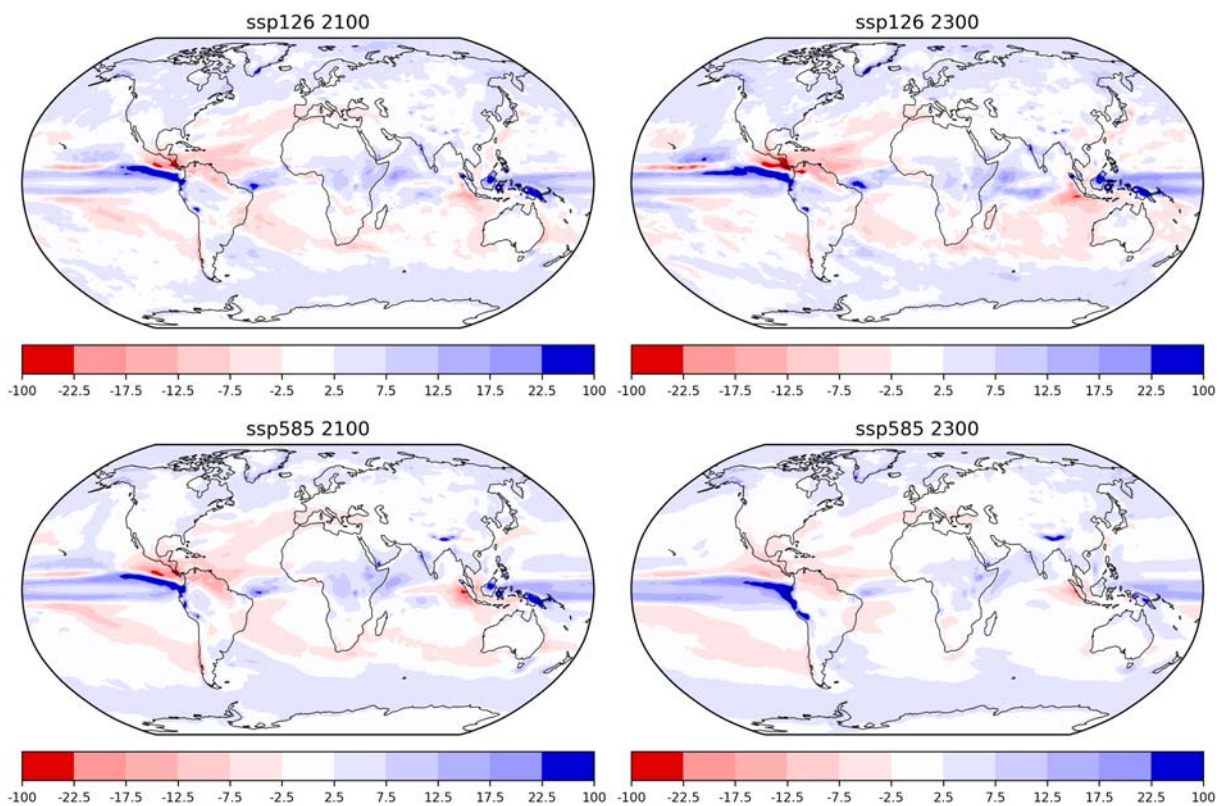
Figure 33. Same as Figure 32 but for the relative change in surface precipitation normalized by the global mean surface temperature change (in % °C -1 ).
