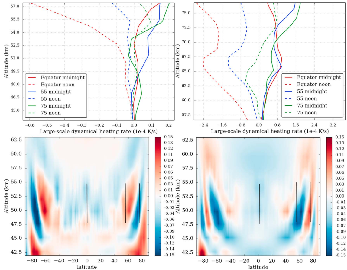
Figure 1. (top row) Vertical profile of the large-scale dynamical heating rate ( 10^{-4} K/s) between 45 and 57 km and from 57 to 75 km. (bottom row) Vertical wind of the Laboratoire de Météorologie Dynamique Venus Global Climate Modeling ( \text{Pa s}^{-1} ) at night (left column) and noon (right column) between 42 and 63 km. Positive value of vertical means downward wind, and positive value means upward wind. The black lines represent the convective activity vertical extension.
