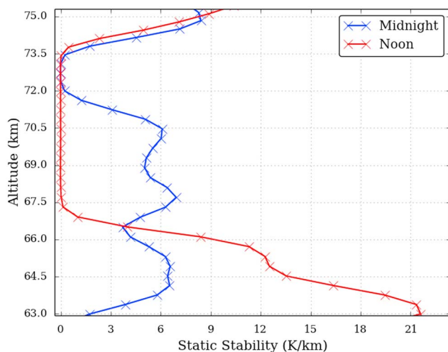
Figure 20. Comparison of the domain-averaged static stability vertical profile ( \text{K/km} ) for equatorial conditions at noon and at midnight between 63 and 75 km.
