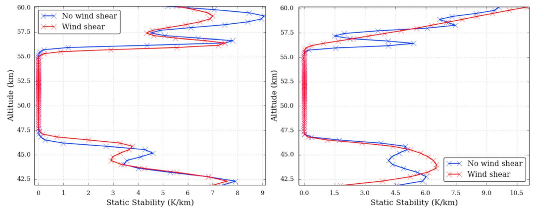
Figure 11. Comparison of the vertical profile of the domain-averaged static stability (K/km) at cloud top between the presence of a wind shear and no wind shear for equatorial condition at midnight (left) and noon (right).
