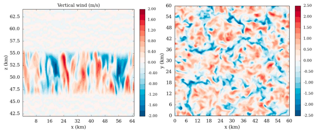
Figure 4. Snapshots of the cloud convective vertical motions: (left) vertical cross section at y = 20 km between 42 and 65 km of altitude and (right) horizontal cross section at 51 km of the vertical wind (m/s) at the equator at noon.
