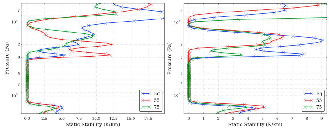
Figure 9. Comparison of the vertical profile of the domain-averaged static stability (K/km) for the equator, 55° and 75° of latitude at noon (left) and midnight (right).
