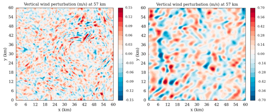
Figure 13. Comparison of two snapshots of the vertical wind perturbation (m/s) at the equator at midnight without (left) and with (right) wind shear.
