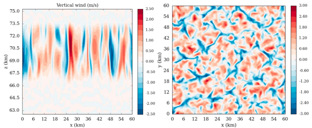
Figure 17. Snapshots of the convective vertical motions: (left) vertical cross section at y = 20 km between 63 and 75 km and (right) horizontal cross section at 51 km of the vertical wind (m/s) for equatorial condition at noon.
