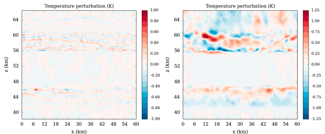
Figure 12. Impact of the wind shear: Comparison of two snapshots of the temperature perturbation (K) at the equator at midnight without (left) and with (right) wind shear.
