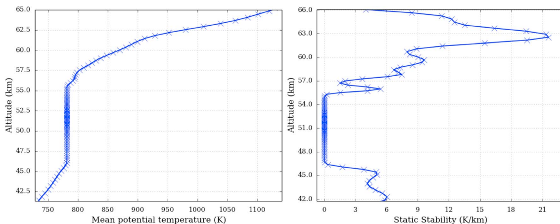
Figure 3. The Venus cloud mixing layer: (left) domain-averaged potential temperature (K) and (right) static stability (K/km) between 42 and 65 km in the equatorial condition at noon.
