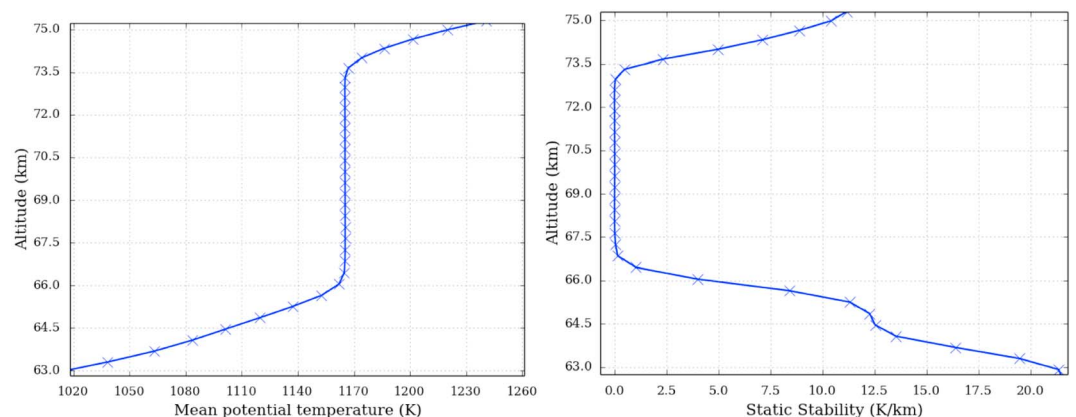
Figure 16. Domain-averaged vertical profile of (left) potential temperature (K) and (right) static stability (K/km) between 63 and 75 km at the equator at noon.
