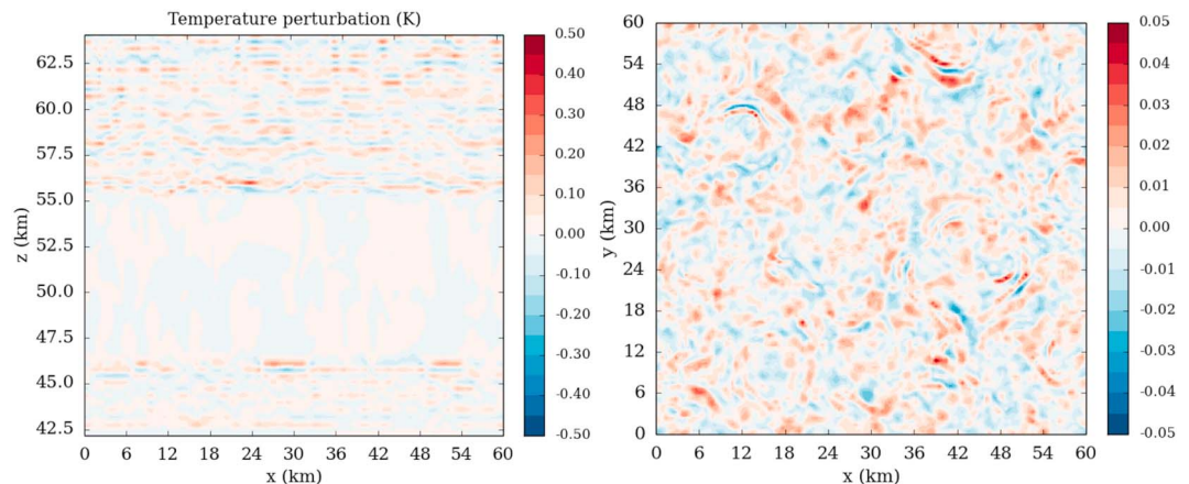
Figure 6. Snapshots of the induced gravity waves: (left) vertical cross section at y = 20 \text{ km} of the temperature perturbation (K) between 42 and 65 km (right) and horizontal cross section at 57 km of the vertical wind perturbation (m/s), at the equator at noon.
