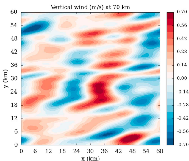
Figure 14. Snapshots of the vertical wind perturbation (m/s) at 70 km at the equator at midnight in presence of wind shear.
