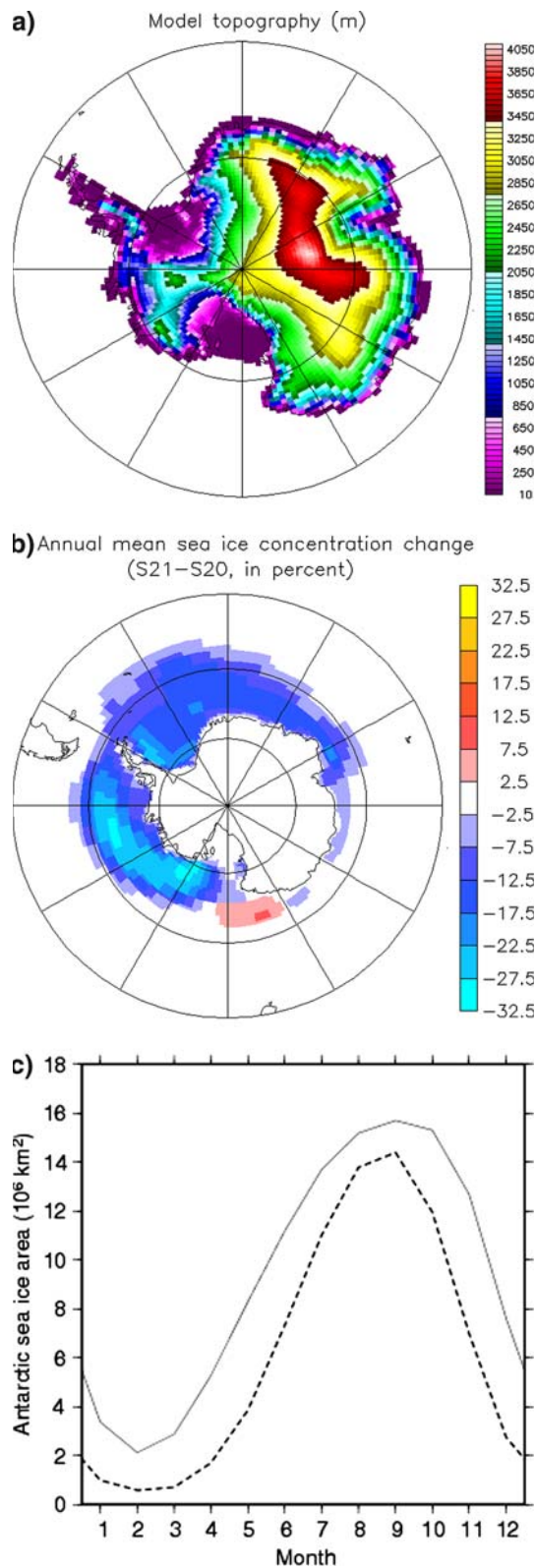
Fig. 1 Model configuration and boundary conditions. a Model topography of the Antarctic continent (m). b Annual mean sea ice concentration change (S21–S20, in percent). c Prescribed Antarctic Sea ice extent for the twentieth century simulations (thin full line: O20; thick dashed line: S20)
