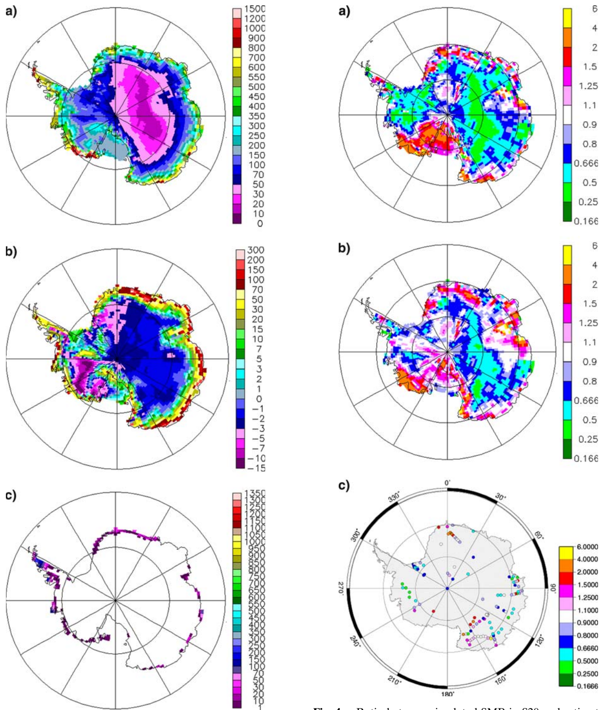
Fig. 3 Individual components of the simulated Antarctic Ice Sheet SMB ( \text{kg m}^{-2} \text{ year}^{-1} ) for the years 1981–2000. a Precipitation; b sublimation; c melt
