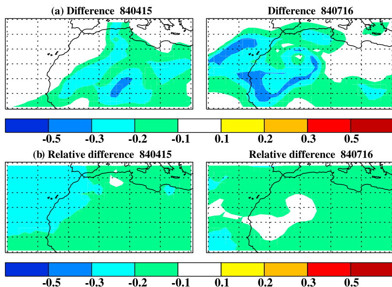
Figure 9. (a) Absolute and (b) relative differences between MS AAI calculated using nadir looking viewing angle and using 45^\circ viewing zenith angle in (left) April and (right) July 1984.
