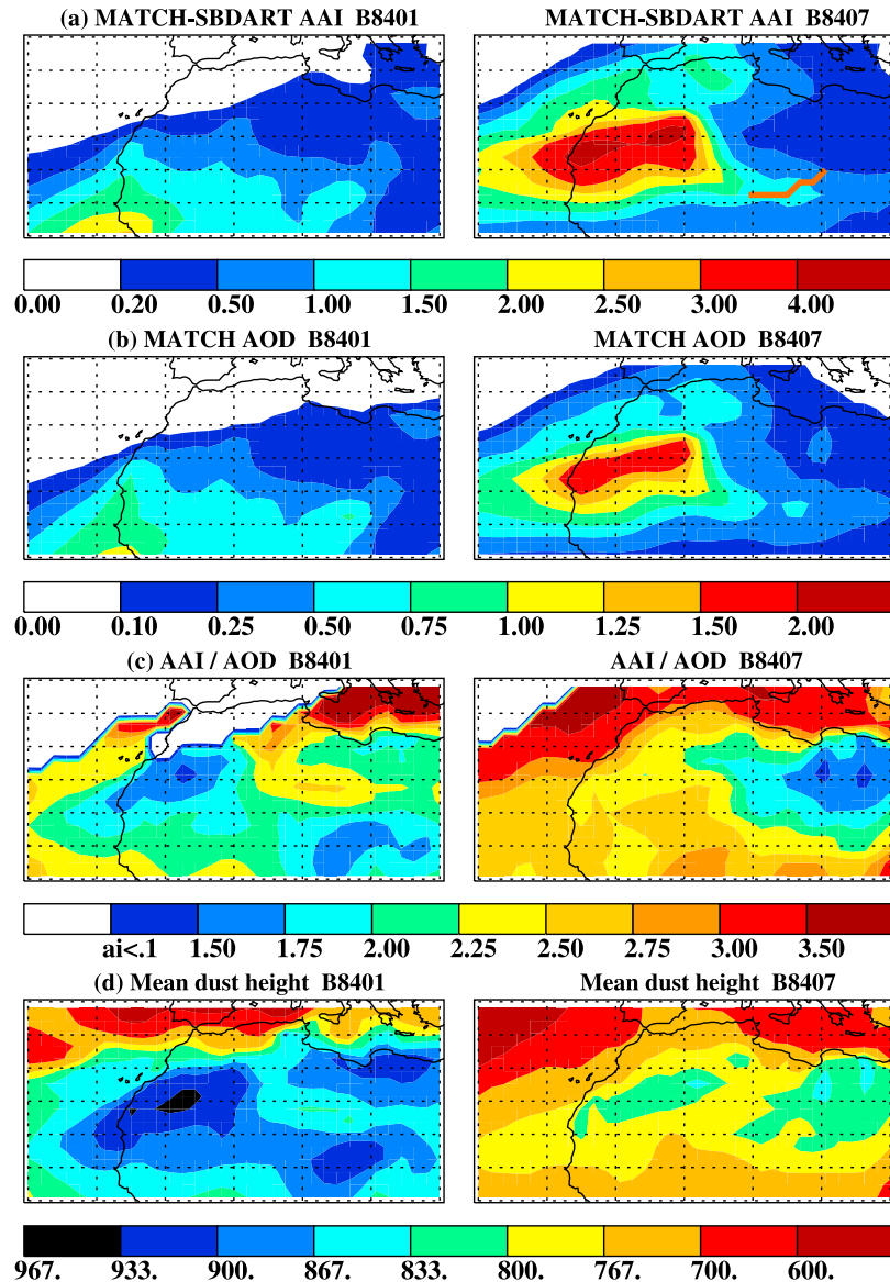
Figure 3. (a) Spatial distributions of simulated AAI, (b) AOD distributions (c), ratios between AAI and AOD, and (d) average height of dust ( \sigma \times 1000 ) for (left) January and (right) July 1984. The pink thick line in Figure 3a (right) shows the location of the cross section shown in Figure 2.
