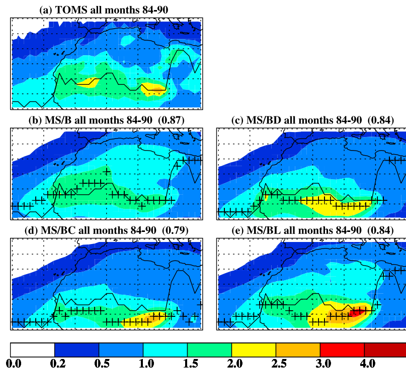
Figure 12. Distributions of AAI averaged over all months and years from (a) TOMS observation and (b) MS/B (MATCH-SBDART case B), (c) MS/BD, (d) MS/BC, and (e) MS/BL simulations. The solid line and pluses show the latitudes at which TOMS and MS AAI, respectively, maximize on each longitude. Numbers in parentheses are correlation coefficients between MS and TOMS AAI.
