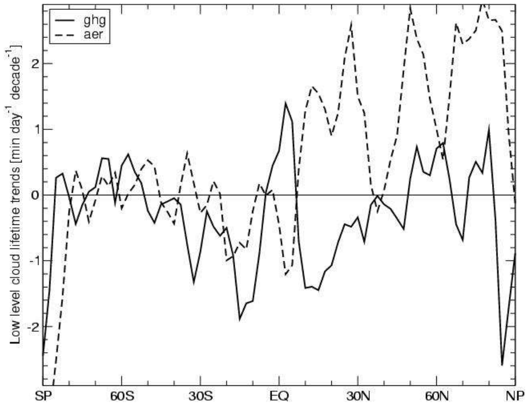
Figure 9: Zonal mean linear trends of the annual mean diurnal lifetime of low-level clouds (min day -1 decade -1 ). Differences between scenarios are shown as in Fig. 4.
