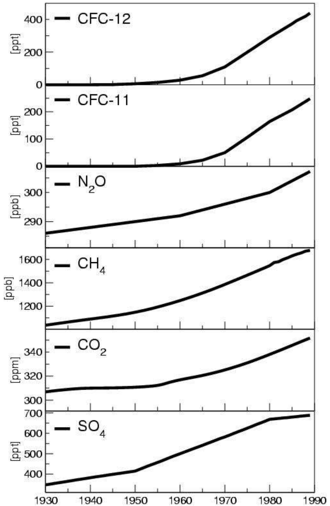
Figure 1: The evolution of the sulfate aerosol mass concentration (850 hPa, Boucher and Pham, 2001) and greenhouse gas (Myhre et al., 2001) concentrations. Global and annual means are shown.
