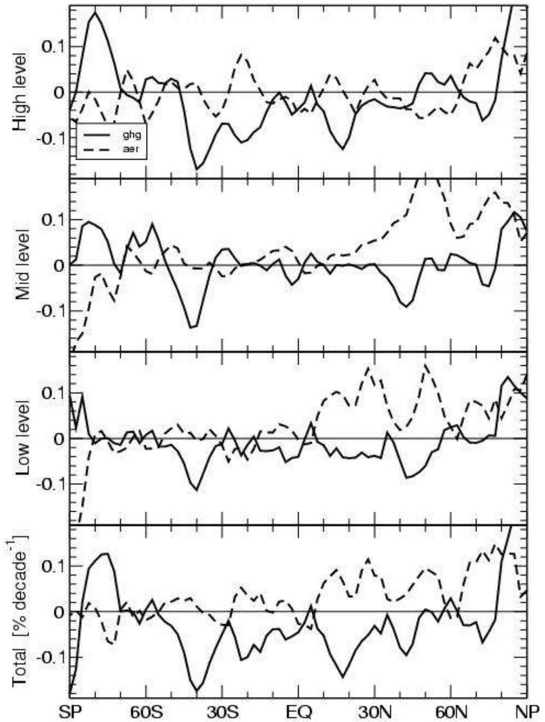
Figure 7: Zonal mean of the linear trends in the annual mean high level, low level, and total cloudiness. The differences between ensemble means are shown, as in Fig. 4.
