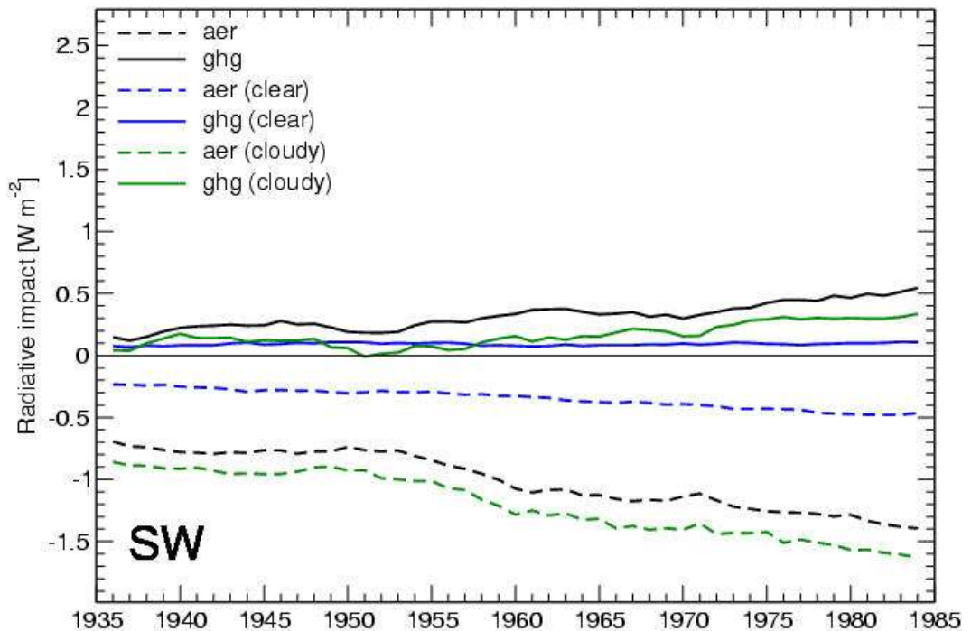
Figure 5: Global annual means of the shortwave radiative impacts ( \text{Wm}^{-2} , as defined in section 2.4.2), for aerosols and greenhouse gases. An 11-year running mean is applied.
