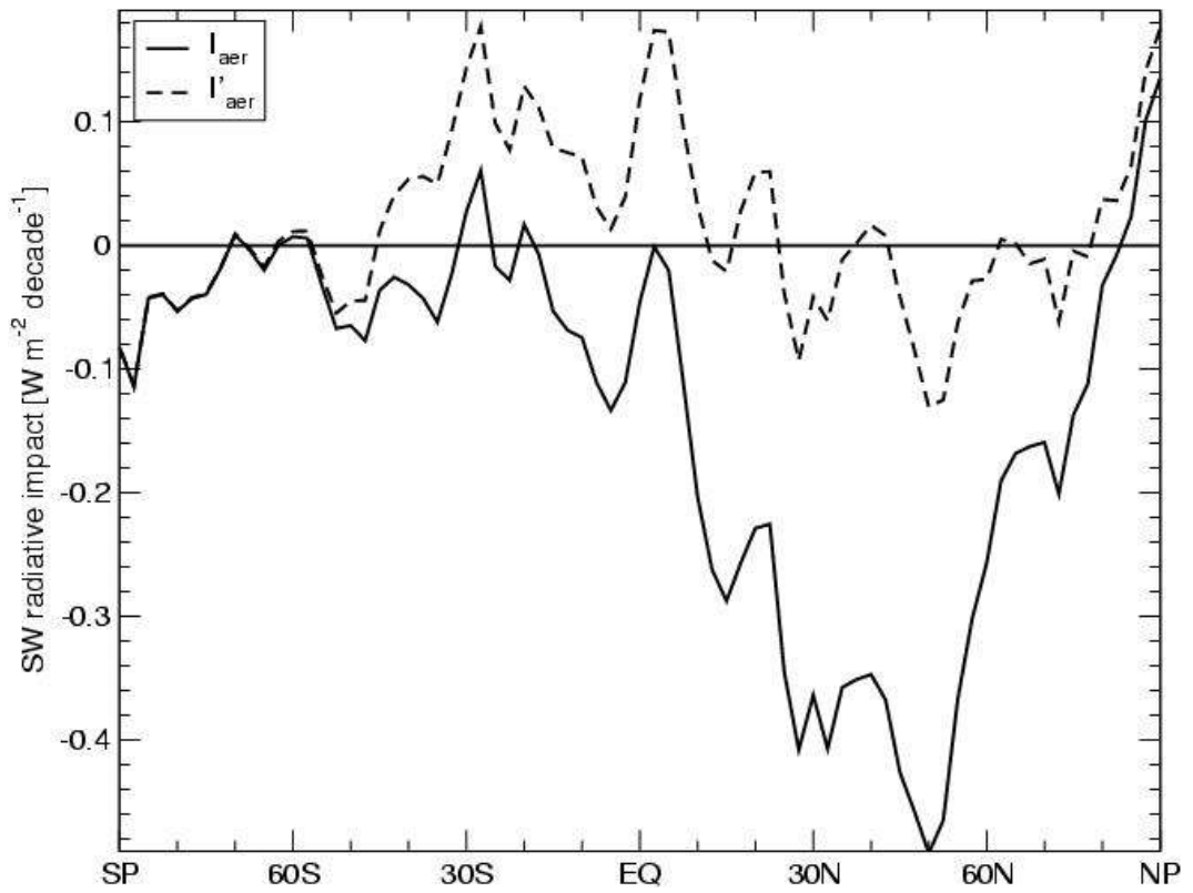
Figure 8: Zonal mean linear trends in the annual mean SW radiative impact of the aerosols as defined in section 2.4.2 ( I_{aer} , solid line) together with the radiative impact of second AIE and cloud feedbacks ( I'_{aer} , dashed line).
