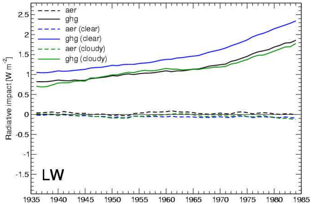
Figure 4: Global annual means of the change in total greenhouse effect (GHE) ( \text{Wm}^{-2} , as defined in section 2.4.1), for aerosols and greenhouse gases, for all-sky (black), cloud-free (blue) and cloud covered (green) conditions. An 11-year running mean is applied.
