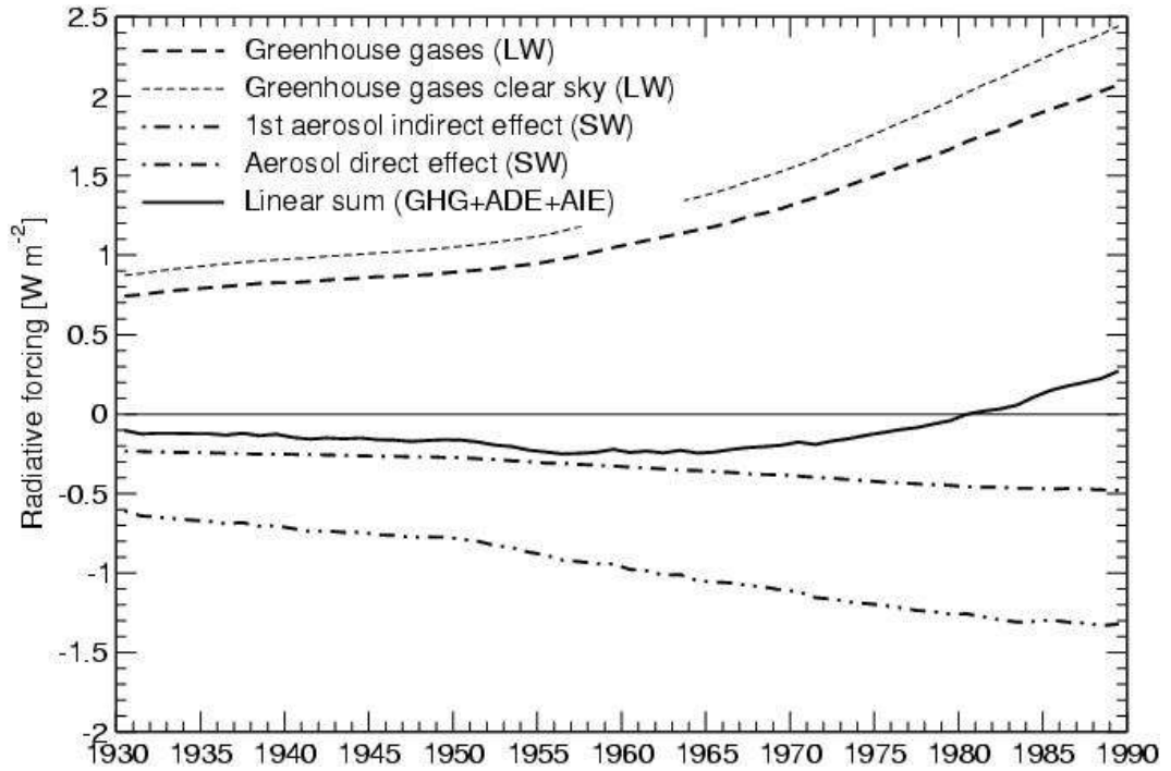
Figure 3: Annual global mean radiative forcings [ \text{Wm}^{-2} ] as diagnosed in the ensemble mean of the GHG+AER simulations: greenhouse gas forcing (LW spectrum, dashed line), aerosol direct forcing (SW spectrum, dot-dashed), and first aerosol indirect forcing (SW, dot-dot-dashed). The solid line corresponds to the sum of the three diagnosed radiative forcings.
