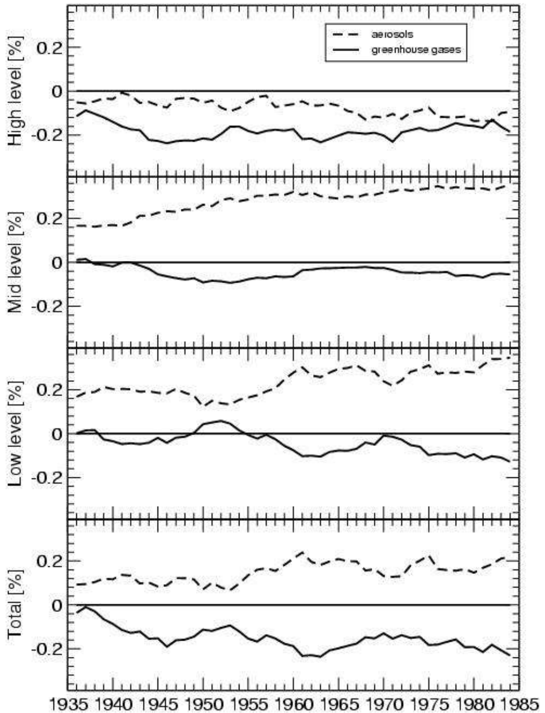
Figure 6: Temporal evolution of the annual and global mean cloudiness. The differences between ensemble means are shown. The evolution for high level (above 450 hPa), mid level (between 800 hPa and 450 hPa), and low level clouds (below 800 hPa), and the total cloudiness is shown. An 11-year running mean is applied.
