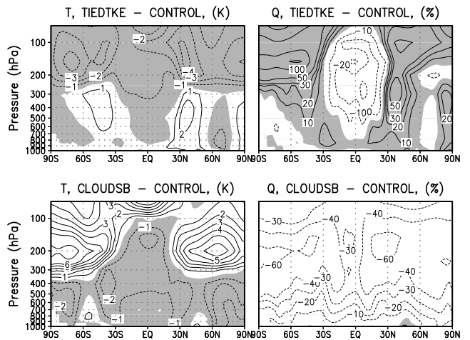
Figure 7: Impact of the convection (TIEDTKE, top) and cloud scheme (CLOUDSB, bottom) on the January mean temperature (left, difference between the sensitivity run and CONTROL) and specific humidity (right, relative difference between the sensitivity run and CONTROL in %). We use log pressure on the vertical in order to focus on the tropopause level. The shaded area correspond to a colder (left) and wetter (right) atmosphere in the sensitivity experiment.
