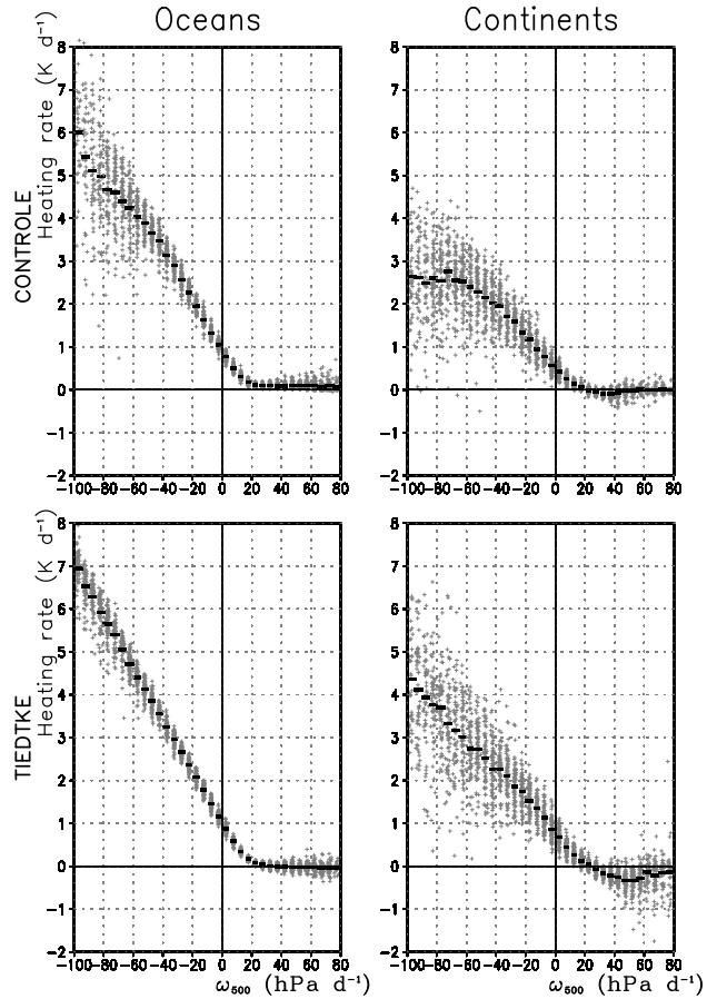
Figure 15: Scatter plot of the convective heating rate ( \text{K d}^{-1} ) at the 550 hPa pressure level, as a function of \omega_{500} ( \text{hPa d}^{-1} ).
