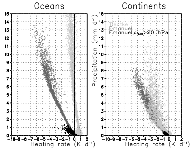
Figure 18: Scatter plot of the convective heating rate at the lowest model level and of the surface precipitation over ocean (left) and continent (right) for the Tiedtke's scheme (light grey crosses), and for the Emanuel's scheme (dark grey: no selection, black: \omega_{500} > 20 \text{ hPa} ).
