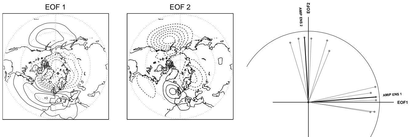
Figure 5: Leading 2 EOF of monthly wintertime northern hemisphere ERA40 SLP, 1980-2001 (Contours every 1hPa) and projections (area-weighted correlations) of the EOF of the different simulations on the phase space defined by the two EOFs. For reference, a circle of radius unity is plotted. Thin lines are individual simulations, the thick lines are for the ensemble.
