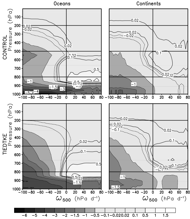
Figure 16: Convective moistening ( \text{g kg}^{-1} \text{d}^{-1} ) with same conventions as in Fig. 14. Note that the contouring is refined around 0.
