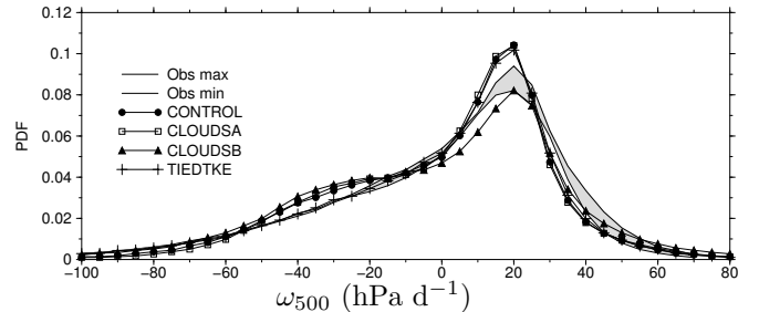
Figure 13: Probability distribution function of \omega_{500} in the 30S-30N latitude band over oceans for two sets of reanalysis (ERA40 and NCEP2 giving rise to the grey area) and for the CONTROL, CLOUDSA/B and TIEDTKE experiments.
