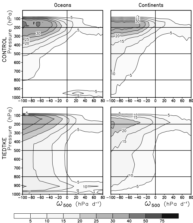
Figure 19: Cloud cover (%) with same conventions as in Fig. 14.
