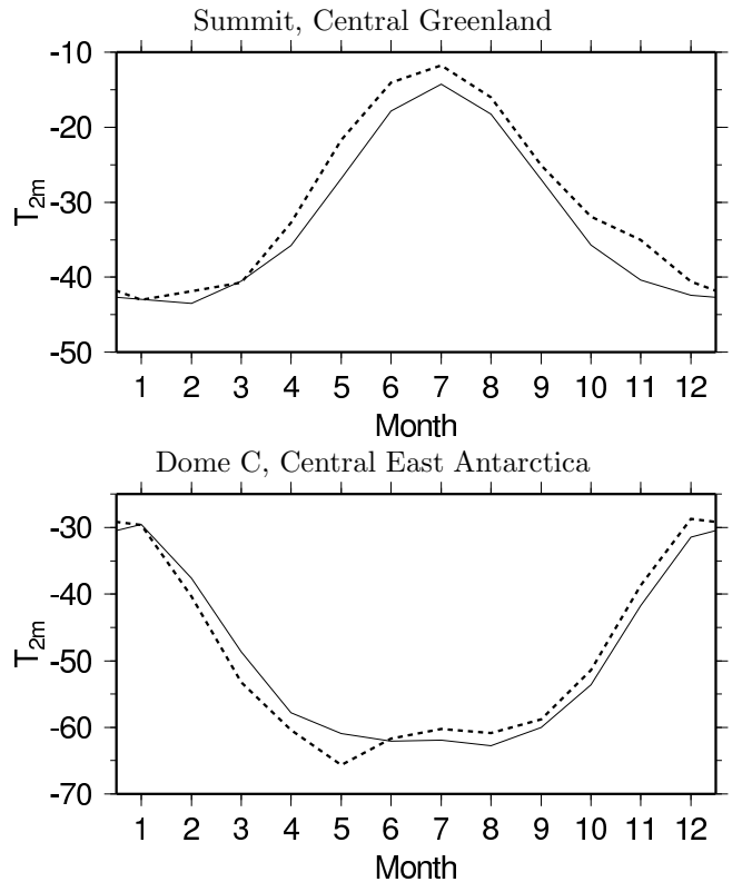
Figure 6: Monthly mean surface air temperatures at Summit (38°W, 72°N, 3250 m asl) and Dome C (123°E, 75°S, 3300 m asl) as simulated with LMDZ4 (full curve, AMIP simulation) and observed (dashed).
