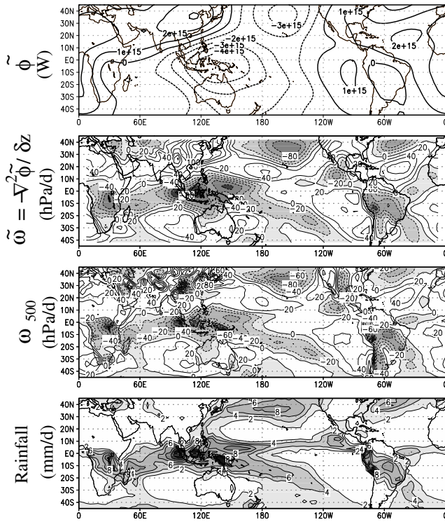
Figure 21: Potential \tilde{\phi} of the annual mean of the horizontal transport of geopotential (upper panel) and mean vertical velocity \bar{\omega} = \frac{1}{Z_0 - z_s} \int_{z_s}^{Z_0} dz \omega = \frac{-1}{Z_0 - z_s} \nabla^2 \tilde{\phi} (with Z_0 - z_s = 15 km) (second panel) for one of the AMIP simulations; to be compared with \omega_{500} and annual precipitation (two lower panels).
