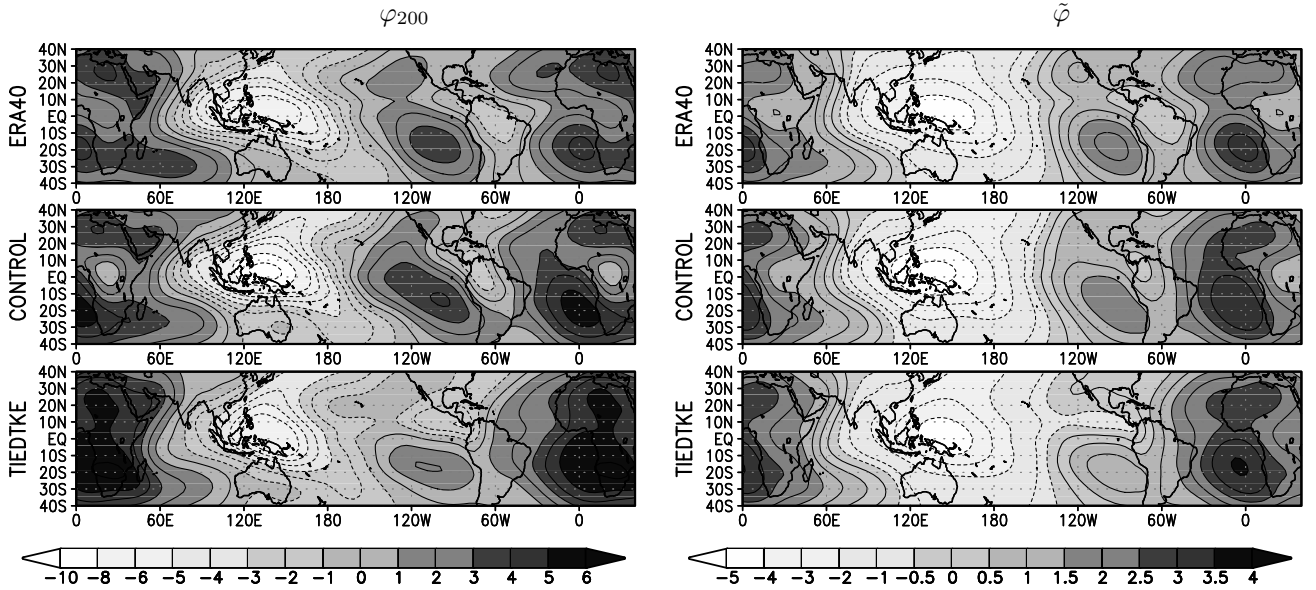
Figure 9: Velocity potential of the wind at 200 hPa ( \varphi_{200} , left, unit 10^6 \text{ m}^2 \text{ s}^{-1} ) and of the z-weighted potential ( \tilde{\varphi} , right, unit 10^{15} \text{ W} ); annual mean for the 1980-2002 period for ERA40 and for a 6-year average for CONTROL and TIEDTKE simulations.
