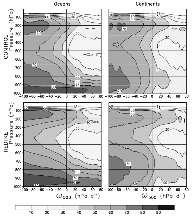
Figure 17: Relative humidity (%) with same conventions as in Fig. 14.
