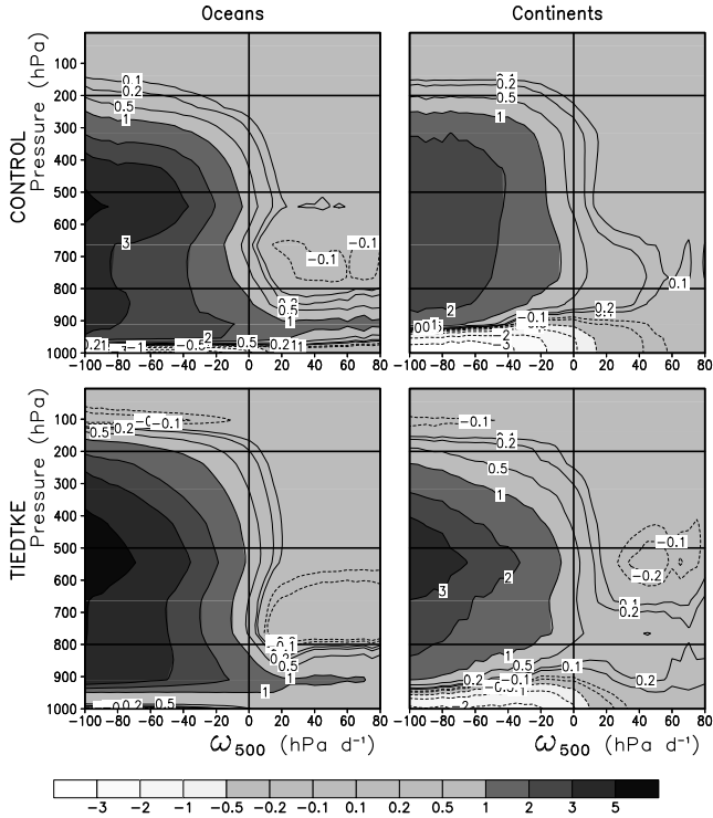
Figure 14: Convective heating rate ( \text{K d}^{-1} ) in a regime sorted diagram (pressure in hPa versus \omega_{500} in \text{hPa d}^{-1} ) for the CONTROL (with Emanuel’s scheme) and TIEDTKE experiments over oceans (left) and continents (right). Note that the contouring is refined around 0.
