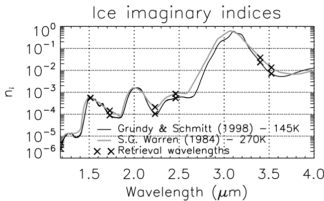
Figure A2. Imaginary indices n_i of hexagonal water ice measured by Grundy and Schmitt [1998] and Schmitt et al. [1998] (black curve) and Warren [1984] (gray curve). The sample temperatures are 145 K and 270 K, respectively. Times symbols indicate the n_i values for the wavelengths used in the retrieval. Ice temperature changes the sharpness of the absorption bands and has a non-negligible effect on the retrieved ice particle sizes.
