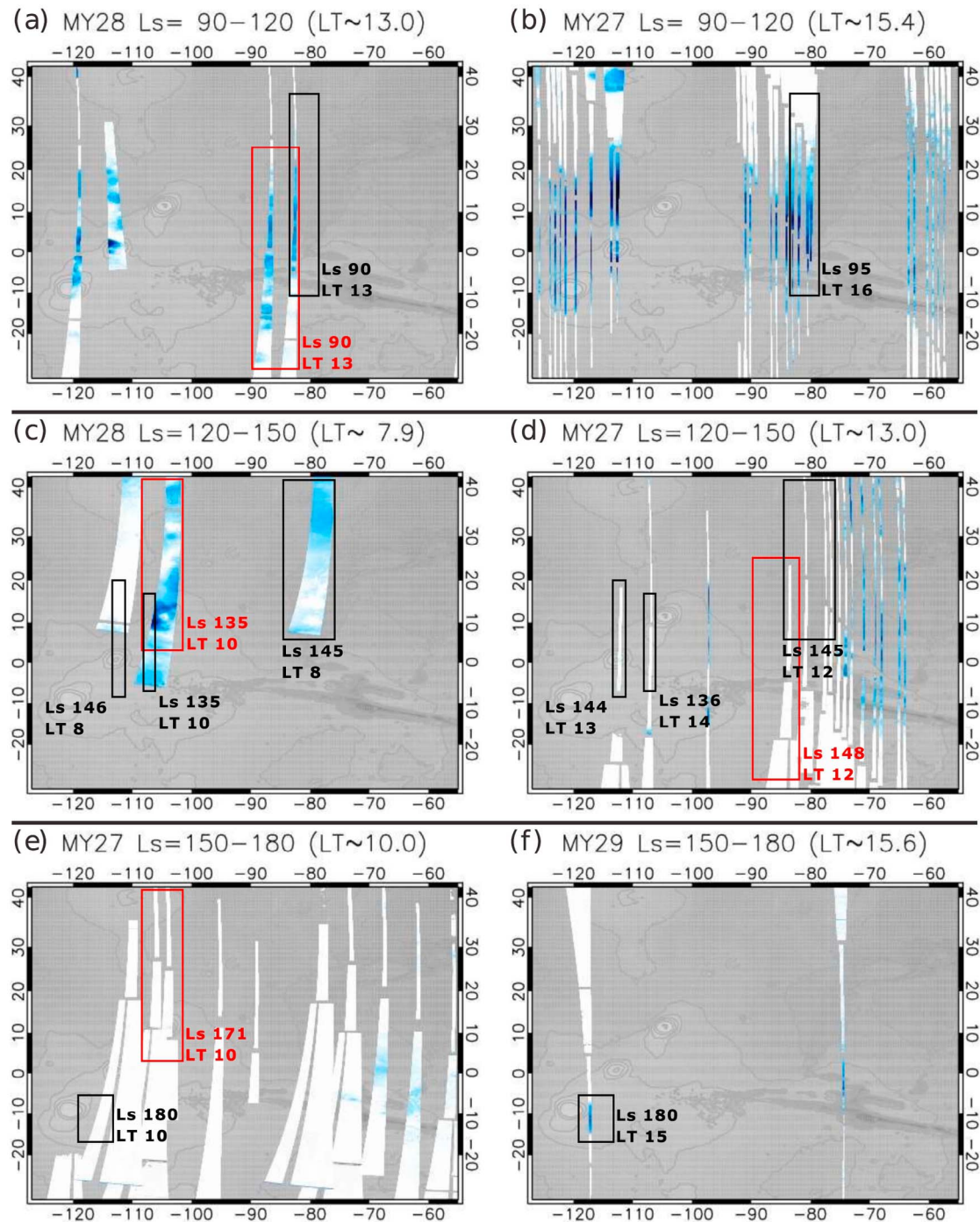
Figure 2. Same as Figure 1 for the (a and b) L_s = 90-120^\circ , (c and d) L_s = 120-150^\circ , and (e and f) L_s = 150-180^\circ periods.
