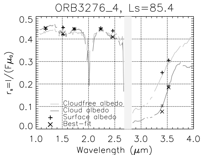
Figure 6. Example of fit obtained for a typical cloud (shown in Figure 7). The cloud-free and cloud spectra measured by OMEGA are shown in light and dark gray, respectively. The 1.5 \mu\text{m} water ice absorption band is clearly seen, whereas the 2 and 3.1 \mu\text{m} bands are reflected by the negative and positive slopes around 2.2 and 3.4 \mu\text{m} , respectively. Plus symbols show the surface albedo obtained after removing the contributions of scattering by the dust layer and thermal emissions. Times symbols represent the final best-fit. Instrumental 1-\sigma error is also given for the cloud spectrum, but can hardly be distinguished, except maybe in the L channel.
